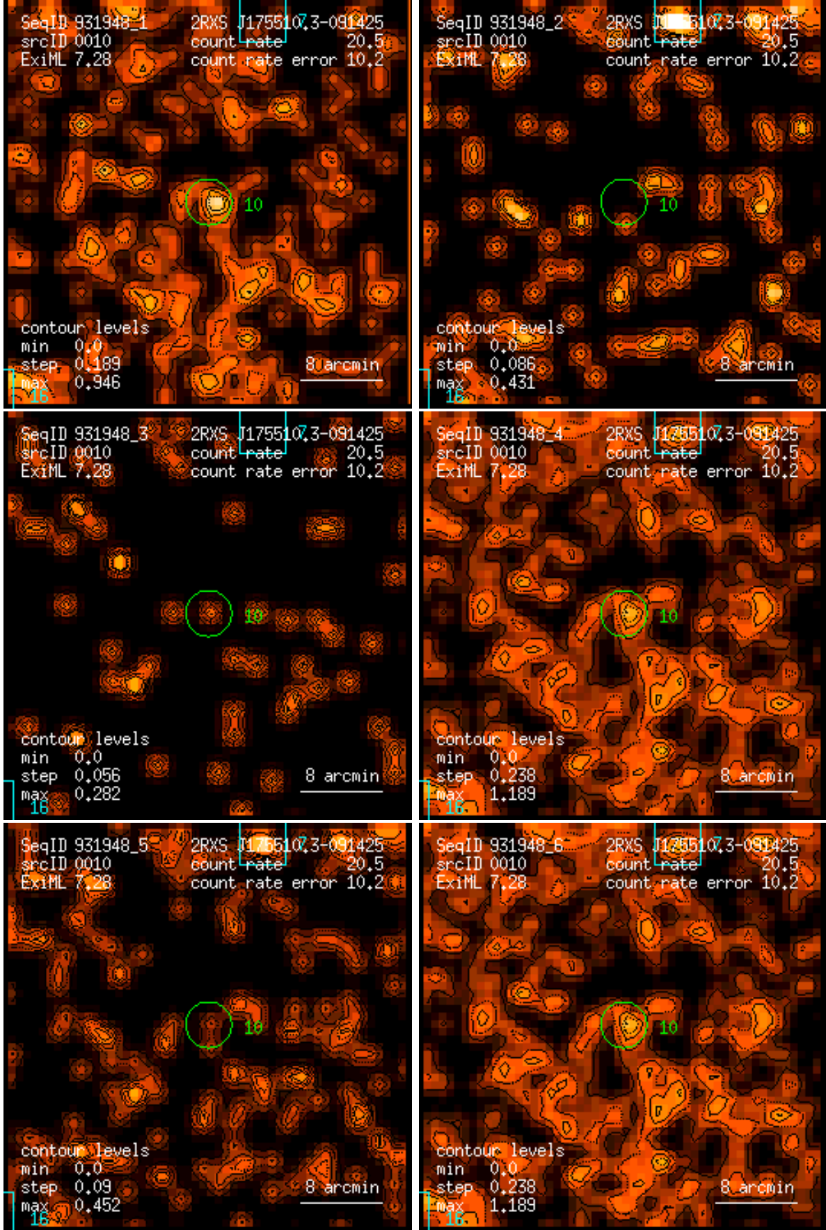
Figure 10: RASS 931948: detection 0010: band rate images, Gaussian filter: (1) PSPC channels 11 – 41, (2) 52 – 90, (3) 91 – 201, (4) 11 – 235, (5) 52 – 201, (6) 11 – 201. Broad band rates in counts/ks. Band rate contour levels in counts/ks/arcmin 2 .
