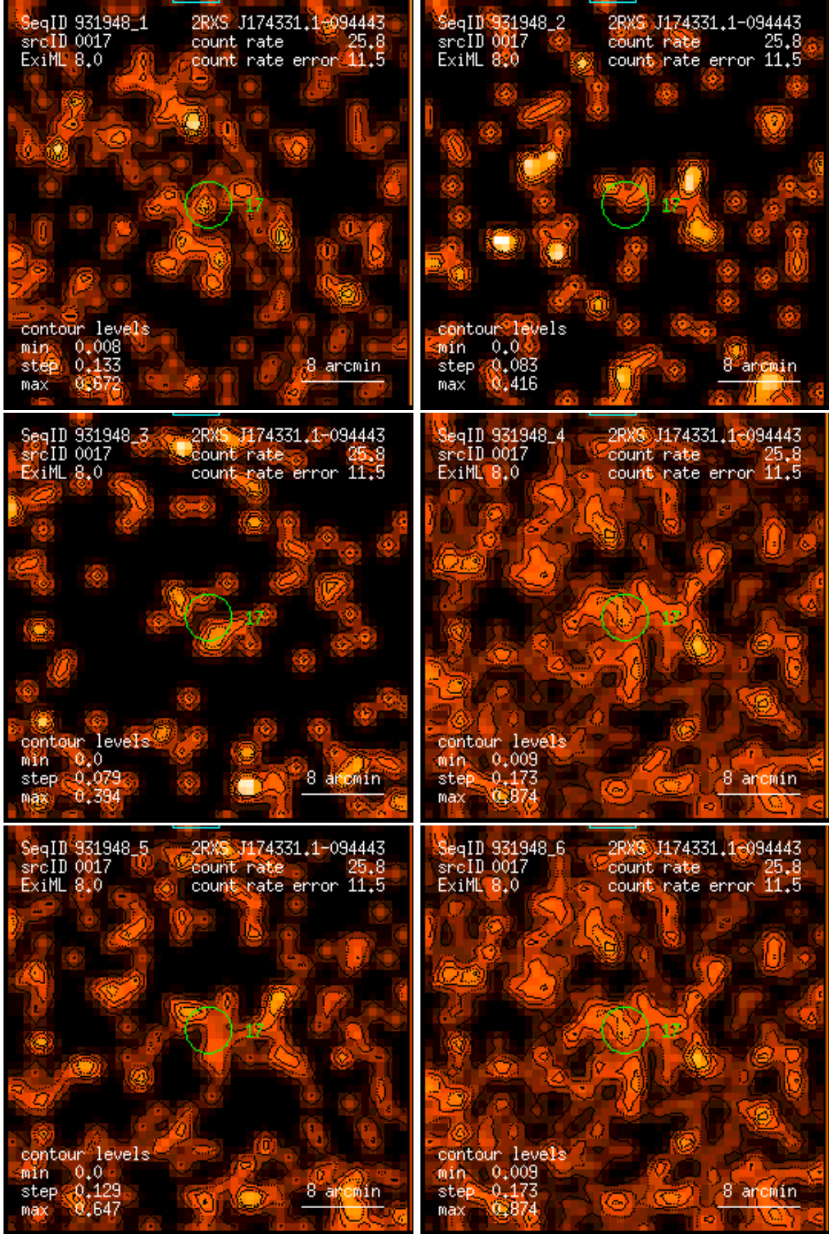
Figure 17: RASS 931948: detection 0017: band rate images, Gaussian filter: (1) PSPC channels 11 – 41, (2) 52 – 90, (3) 91 – 201, (4) 11 – 235, (5) 52 – 201, (6) 11 – 201. Broad band rates in counts/ks. Band rate contour levels in counts/ks/arcmin 2 .
