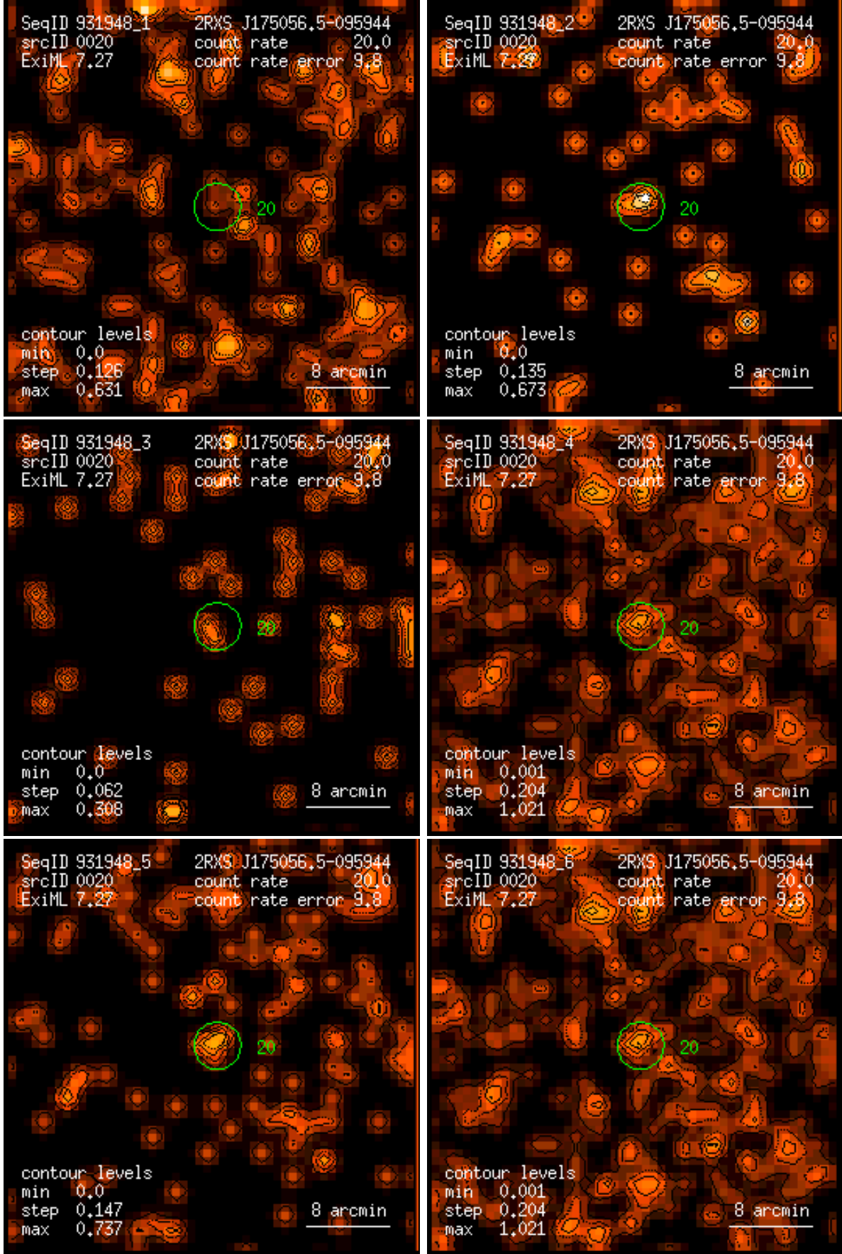
Figure 20: RASS 931948: detection 0020: band rate images, Gaussian filter: (1) PSPC channels 11 – 41, (2) 52 – 90, (3) 91 – 201, (4) 11 – 235, (5) 52 – 201, (6) 11 – 201. Broad band rates in counts/ks. Band rate contour levels in counts/ks/arcmin 2 .
