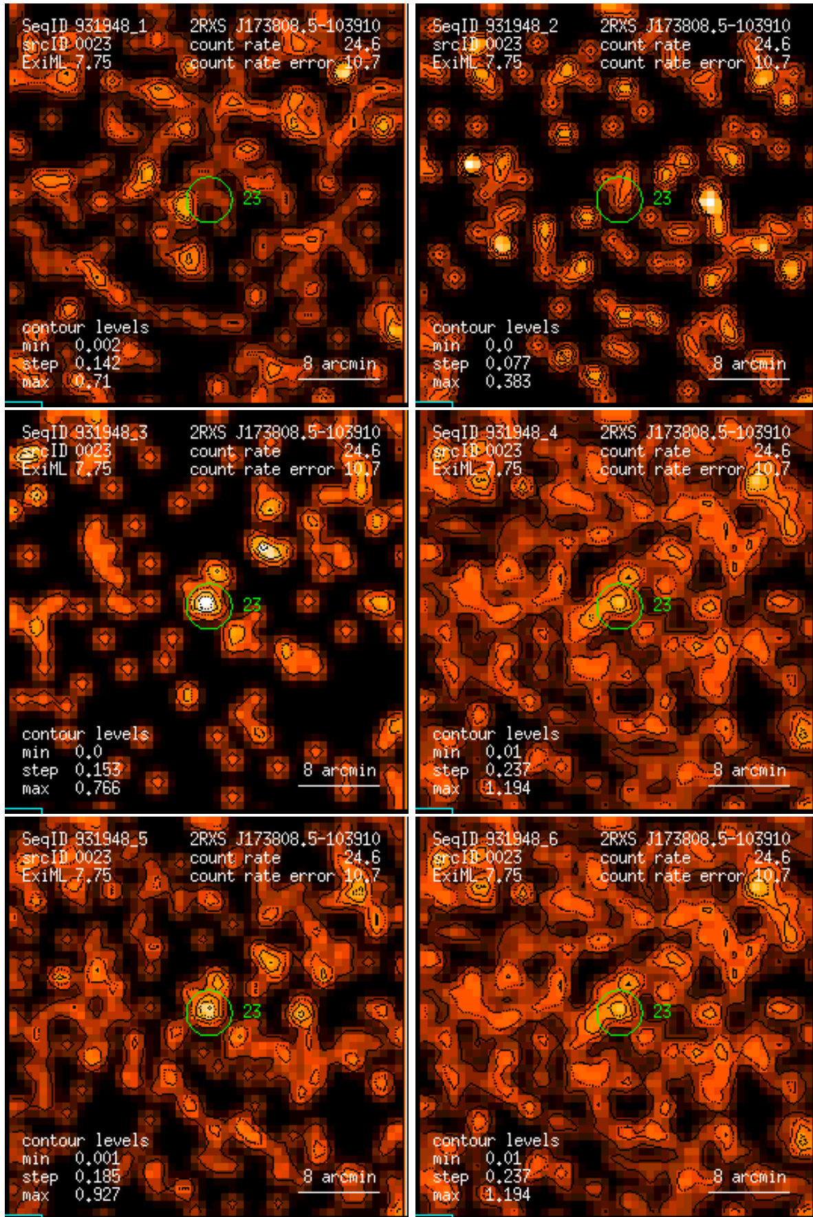
Figure 23: RASS 931948: detection 0023: band rate images, Gaussian filter: (1) PSPC channels 11 – 41, (2) 52 – 90, (3) 91 – 201, (4) 11 – 235, (5) 52 – 201, (6) 11 – 201. Broad band rates in counts/ks. Band rate contour levels in counts/ks/arcmin 2 .
