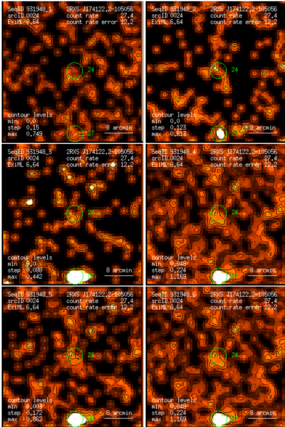
Figure 24: RASS 931948: detection 0024: band rate images, Gaussian filter: (1) PSPC channels 11 – 41, (2) 52 – 90, (3) 91 – 201, (4) 11 – 235, (5) 52 – 201, (6) 11 – 201. Broad band rates in counts/ks. Band rate contour levels in counts/ks/arcmin 2 .
