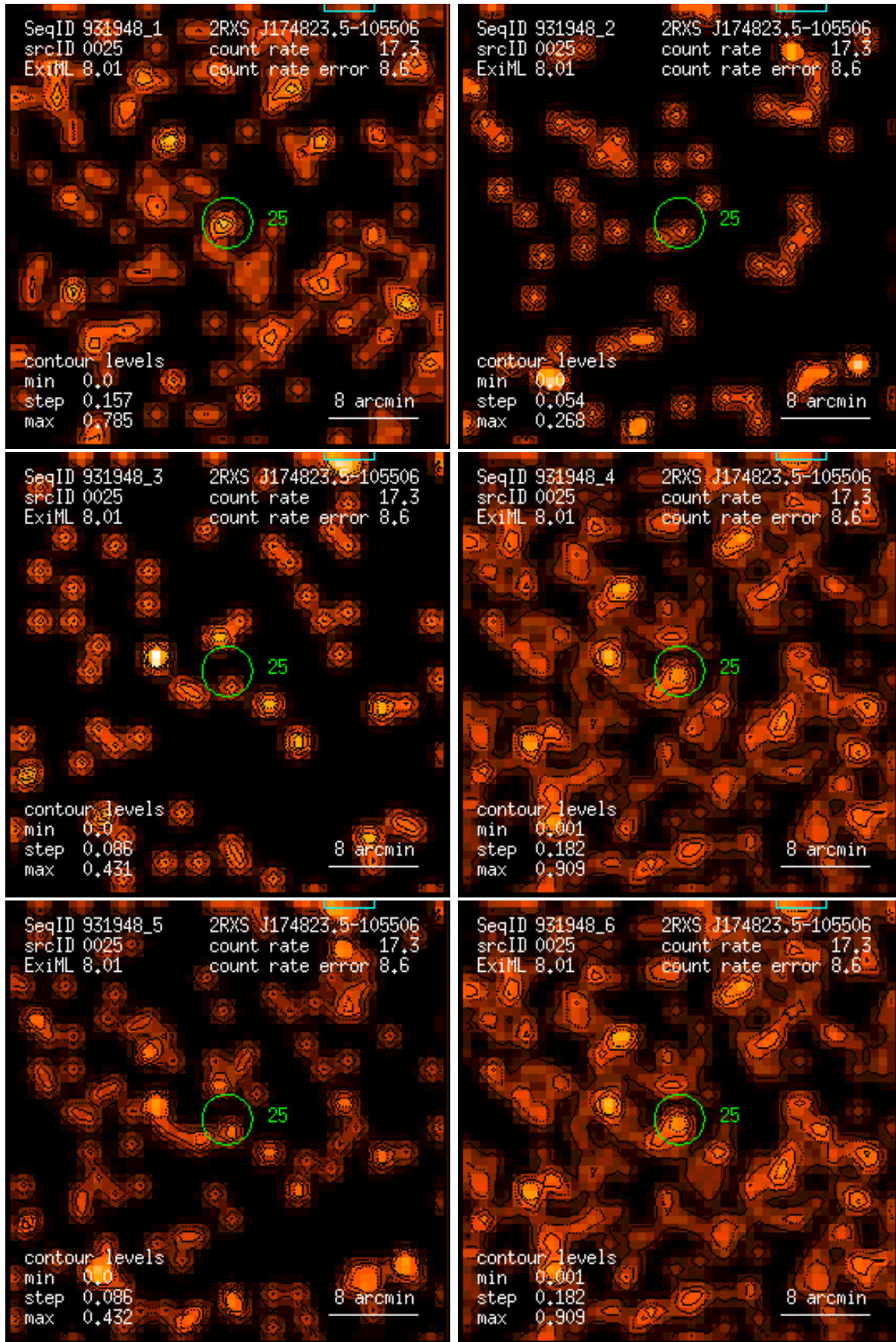
Figure 25: RASS 931948: detection 0025: band rate images, Gaussian filter: (1) PSPC channels 11 – 41, (2) 52 – 90, (3) 91 – 201, (4) 11 – 235, (5) 52 – 201, (6) 11 – 201. Broad band rates in counts/ks. Band rate contour levels in counts/ks/arcmin 2 .
