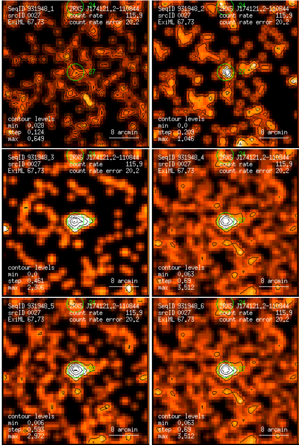
Figure 27: RASS 931948: detection 0027: band rate images, Gaussian filter: (1) PSPC channels 11 – 41, (2) 52 – 90, (3) 91 – 201, (4) 11 – 235, (5) 52 – 201, (6) 11 – 201. Broad band rates in counts/ks. Band rate contour levels in counts/ks/arcmin 2 .
