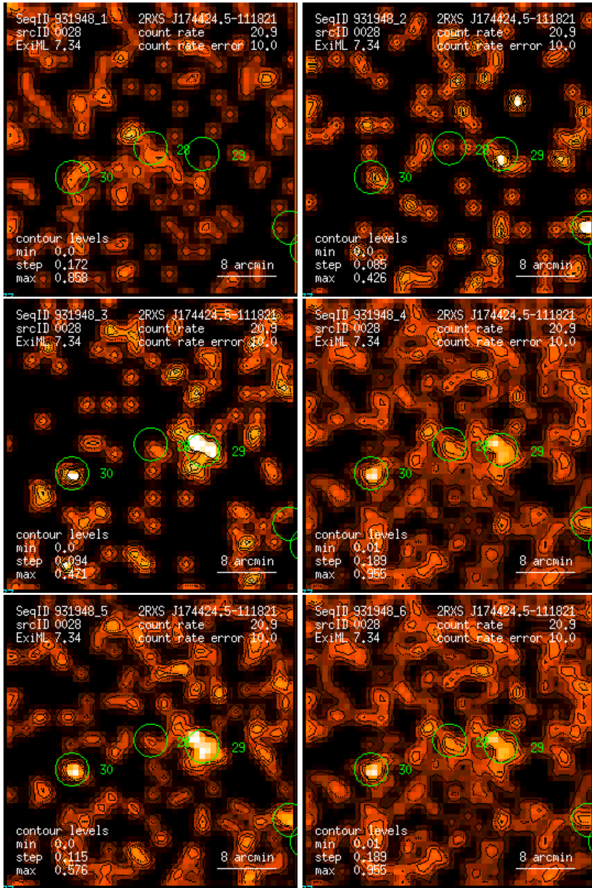
Figure 28: RASS 931948: detection 0028: band rate images, Gaussian filter: (1) PSPC channels 11 – 41, (2) 52 – 90, (3) 91 – 201, (4) 11 – 235, (5) 52 – 201, (6) 11 – 201. Broad band rates in counts/ks. Band rate contour levels in counts/ks/arcmin 2 .
