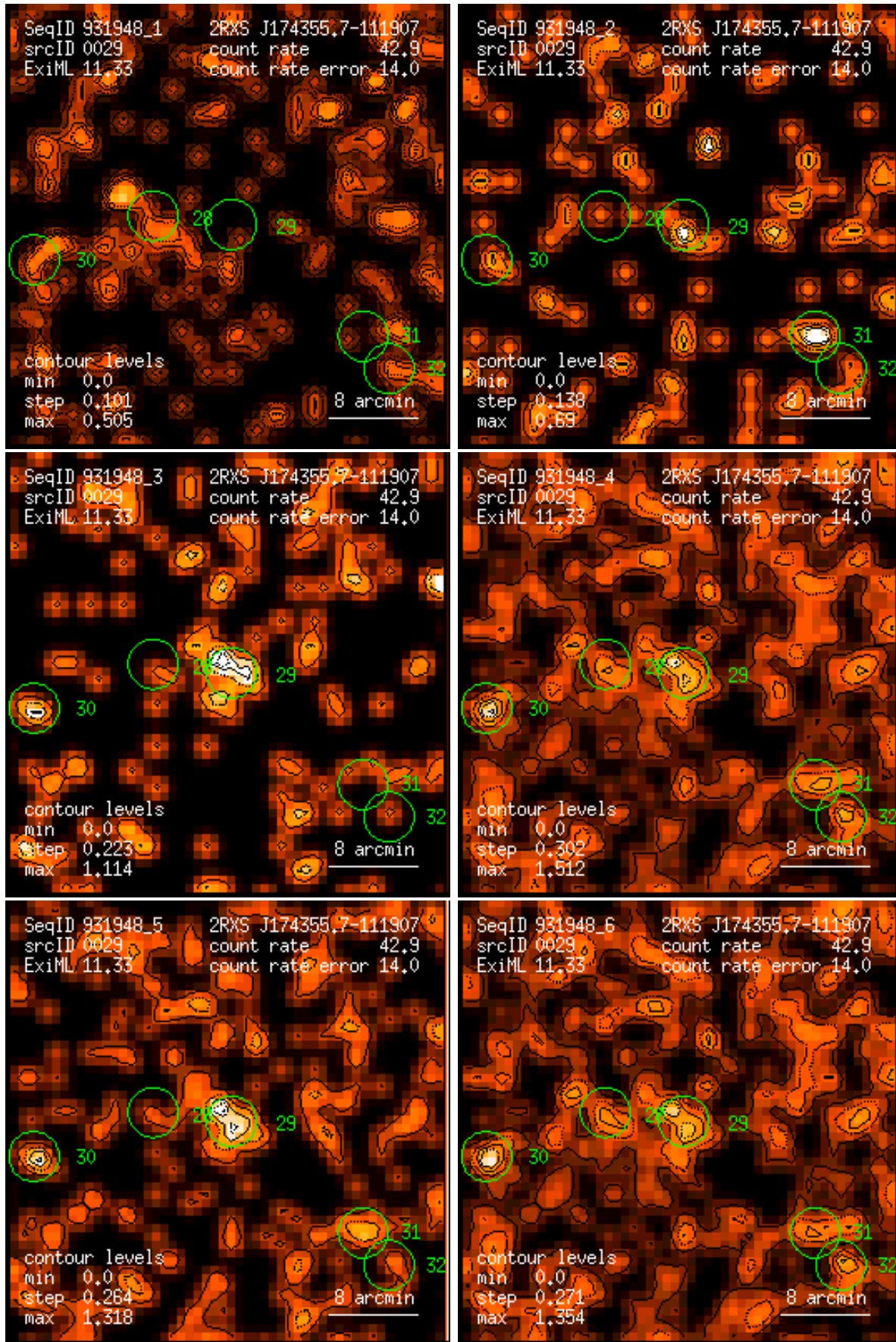
Figure 29: RASS 931948: detection 0029: band rate images, Gaussian filter: (1) PSPC channels 11 – 41, (2) 52 – 90, (3) 91 – 201, (4) 11 – 235, (5) 52 – 201, (6) 11 – 201. Broad band rates in counts/ks. Band rate contour levels in counts/ks/arcmin 2 .
