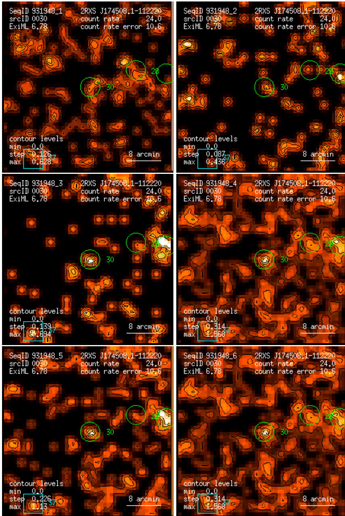
Figure 30: RASS 931948: detection 0030: band rate images, Gaussian filter: (1) PSPC channels 11 – 41, (2) 52 – 90, (3) 91 – 201, (4) 11 – 235, (5) 52 – 201, (6) 11 – 201. Broad band rates in counts/ks. Band rate contour levels in counts/ks/arcmin 2 .
