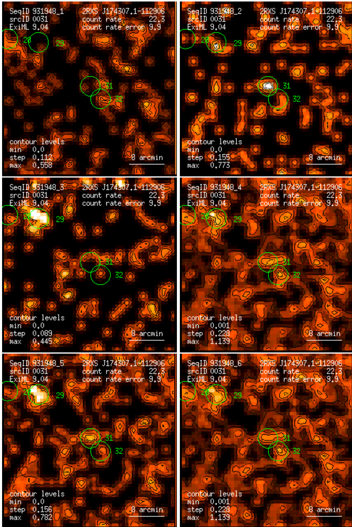
Figure 31: RASS 931948: detection 0031: band rate images, Gaussian filter: (1) PSPC channels 11 – 41, (2) 52 – 90, (3) 91 – 201, (4) 11 – 235, (5) 52 – 201, (6) 11 – 201. Broad band rates in counts/ks. Band rate contour levels in counts/ks/arcmin 2 .
