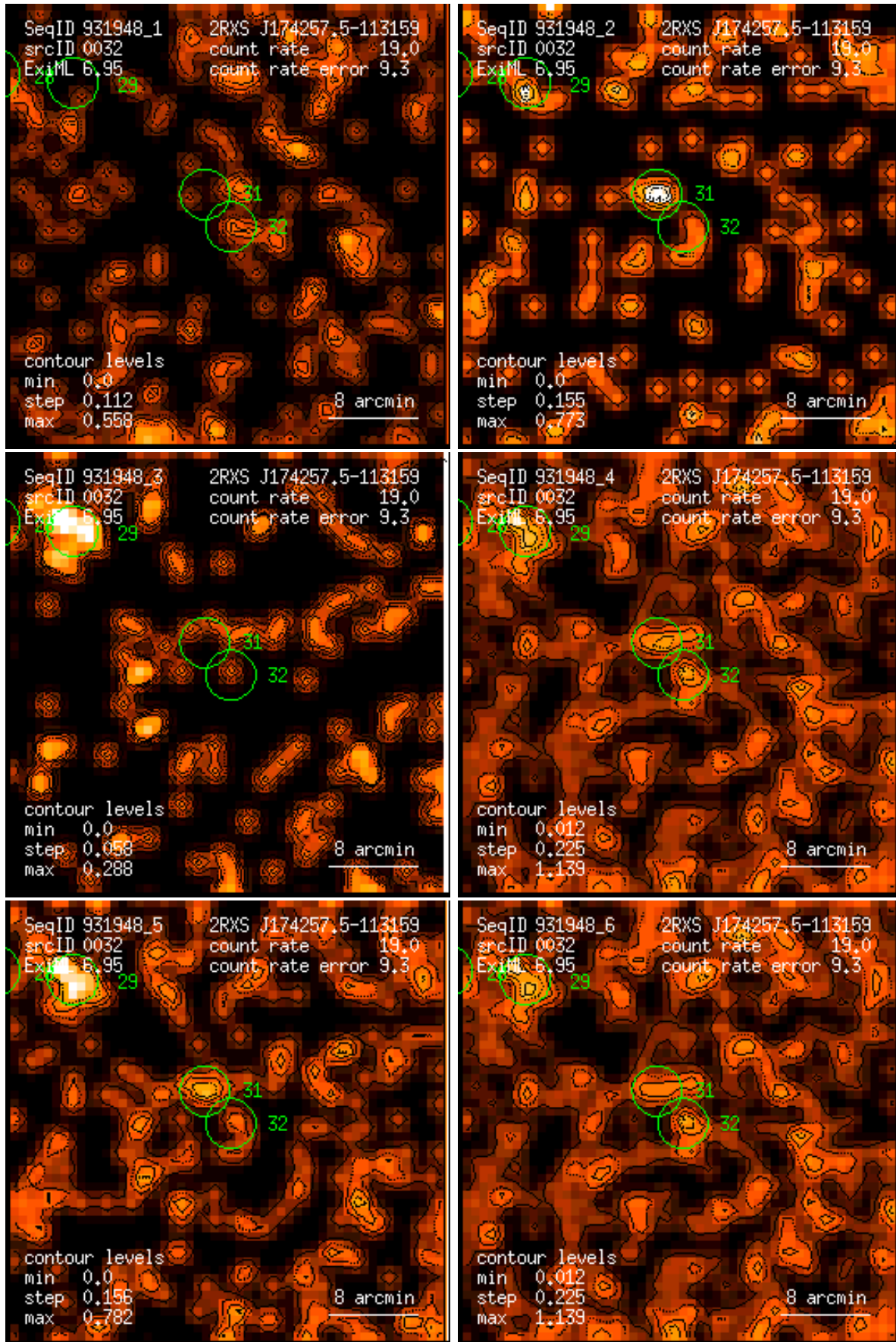
Figure 32: RASS 931948: detection 0032: band rate images, Gaussian filter: (1) PSPC channels 11 – 41, (2) 52 – 90, (3) 91 – 201, (4) 11 – 235, (5) 52 – 201, (6) 11 – 201. Broad band rates in counts/ks. Band rate contour levels in counts/ks/arcmin 2 .
