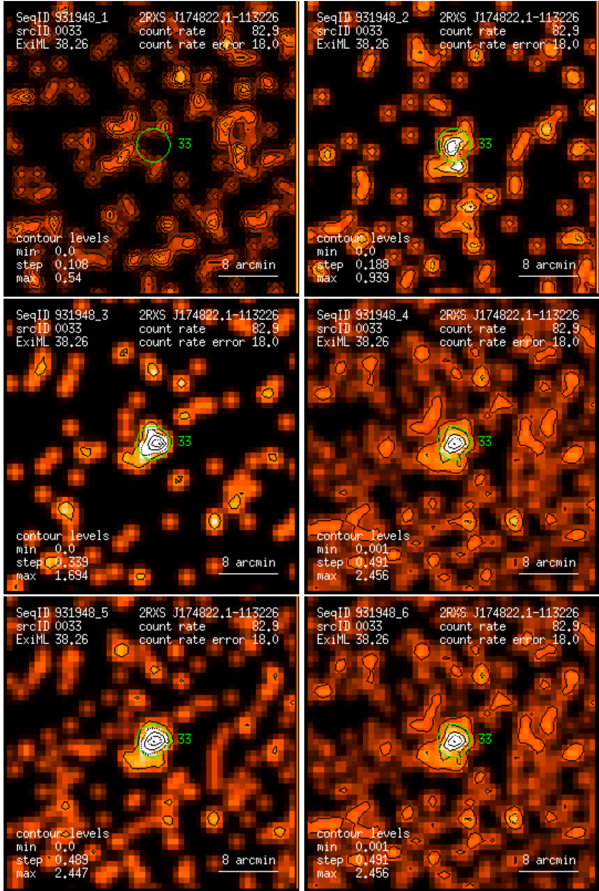
Figure 33: RASS 931948: detection 0033: band rate images, Gaussian filter: (1) PSPC channels 11 – 41, (2) 52 – 90, (3) 91 – 201, (4) 11 – 235, (5) 52 – 201, (6) 11 – 201. Broad band rates in counts/ks. Band rate contour levels in counts/ks/arcmin 2 .
