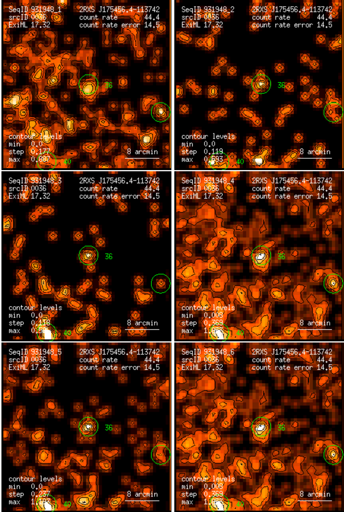
Figure 36: RASS 931948: detection 0036: band rate images, Gaussian filter: (1) PSPC channels 11 – 41, (2) 52 – 90, (3) 91 – 201, (4) 11 – 235, (5) 52 – 201, (6) 11 – 201. Broad band rates in counts/ks. Band rate contour levels in counts/ks/arcmin 2 .
