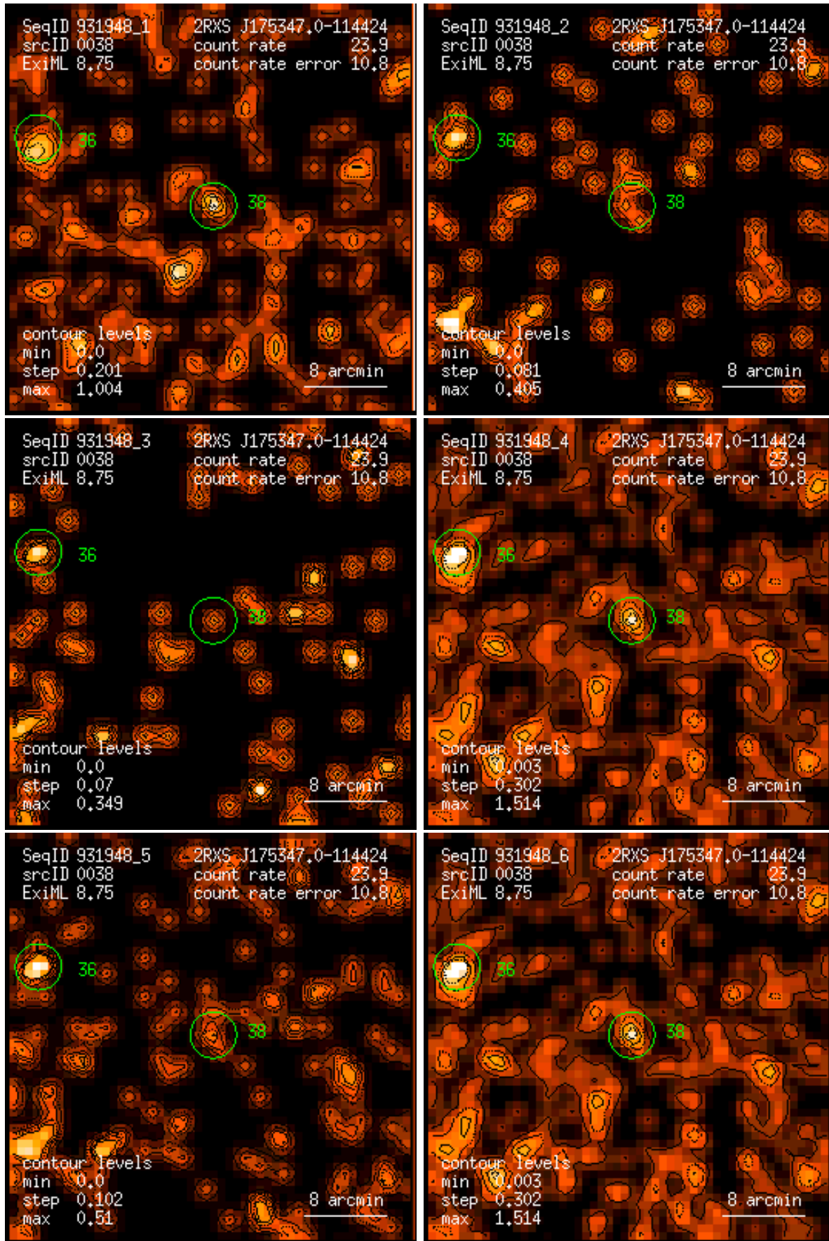
Figure 38: RASS 931948: detection 0038: band rate images, Gaussian filter: (1) PSPC channels 11 – 41, (2) 52 – 90, (3) 91 – 201, (4) 11 – 235, (5) 52 – 201, (6) 11 – 201. Broad band rates in counts/ks. Band rate contour levels in counts/ks/arcmin 2 .
