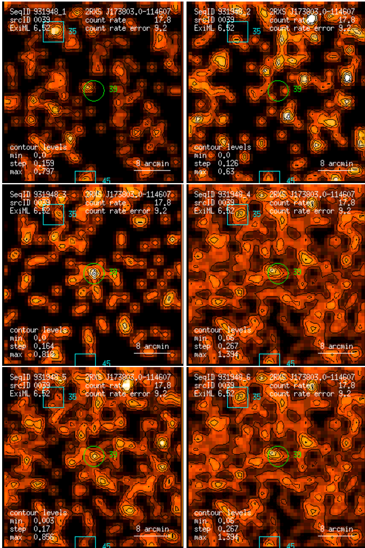
Figure 39: RASS 931948: detection 0039: band rate images, Gaussian filter: (1) PSPC channels 11 – 41, (2) 52 – 90, (3) 91 – 201, (4) 11 – 235, (5) 52 – 201, (6) 11 – 201. Broad band rates in counts/ks. Band rate contour levels in counts/ks/arcmin 2 .
