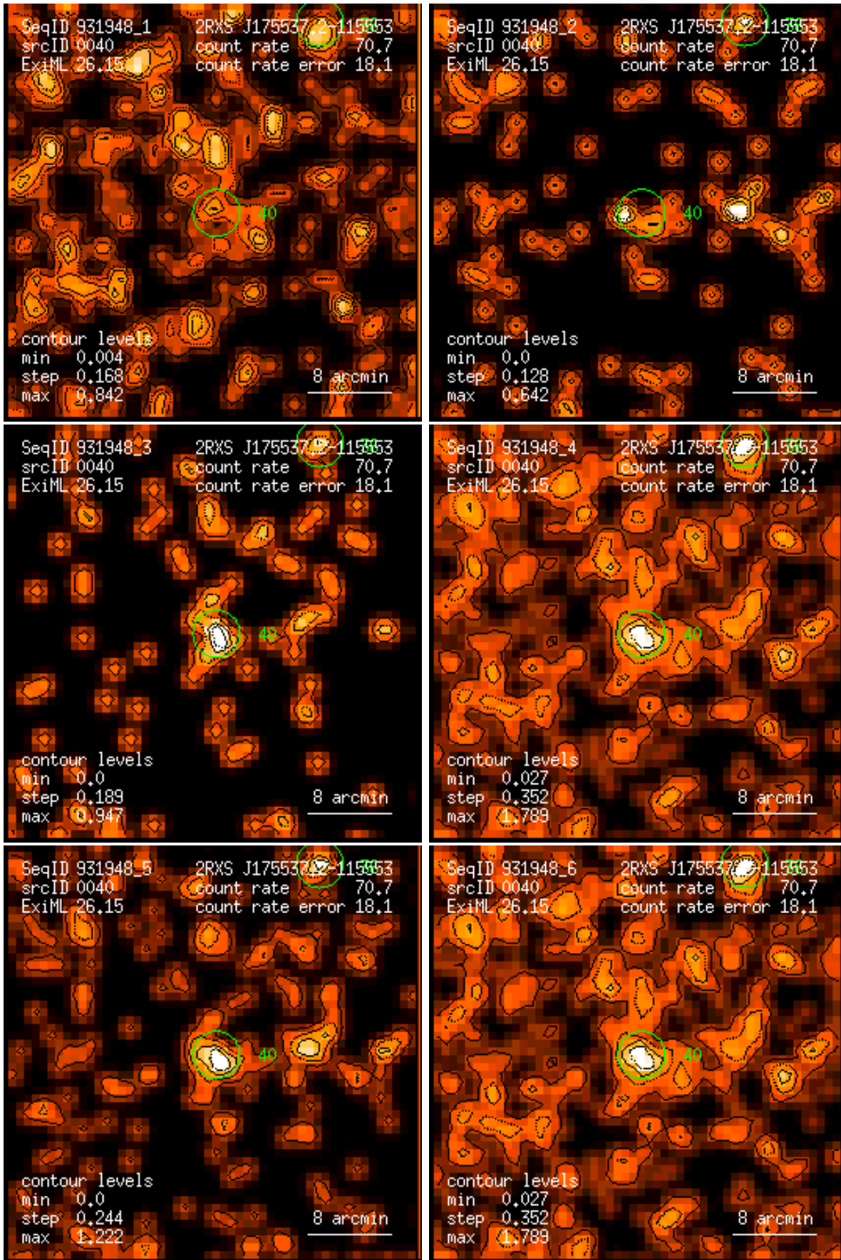
Figure 40: RASS 931948: detection 0040: band rate images, Gaussian filter: (1) PSPC channels 11 – 41, (2) 52 – 90, (3) 91 – 201, (4) 11 – 235, (5) 52 – 201, (6) 11 – 201. Broad band rates in counts/ks. Band rate contour levels in counts/ks/arcmin 2 .
