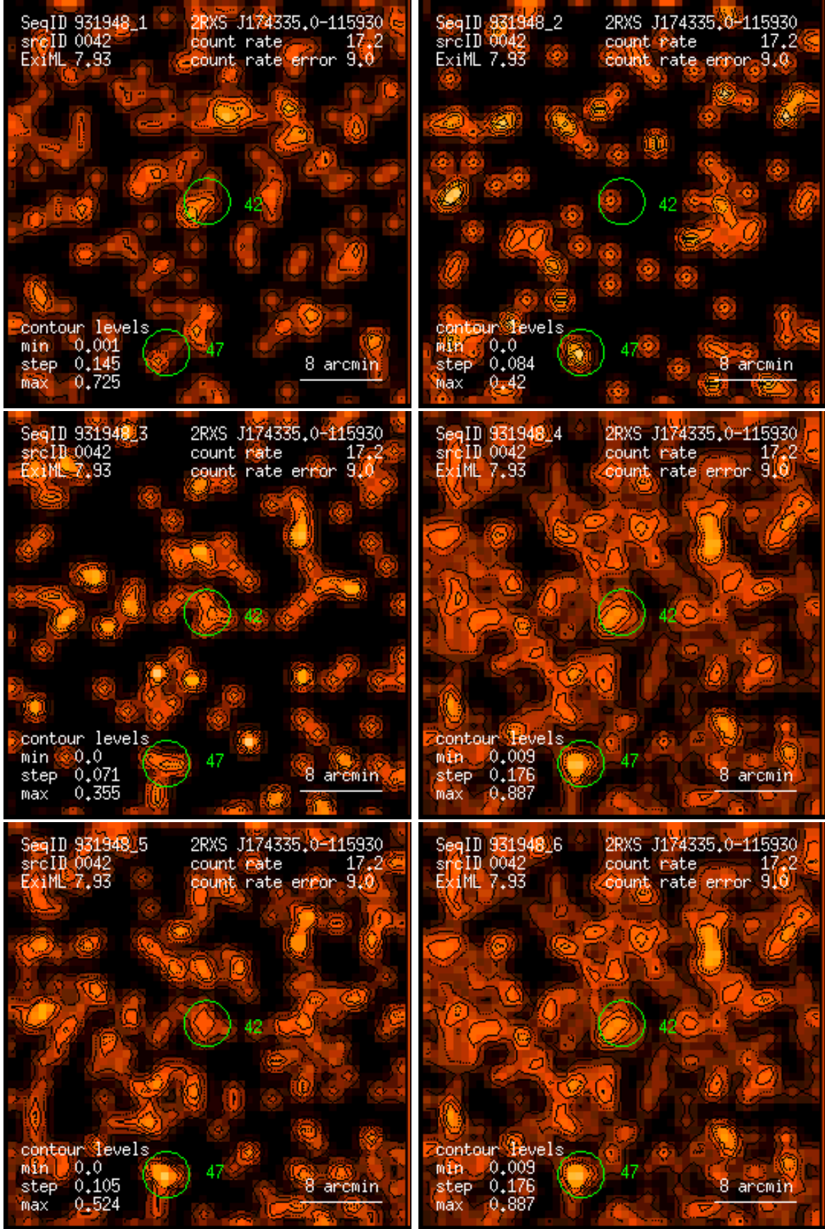
Figure 42: RASS 931948: detection 0042: band rate images, Gaussian filter: (1) PSPC channels 11 – 41, (2) 52 – 90, (3) 91 – 201, (4) 11 – 235, (5) 52 – 201, (6) 11 – 201. Broad band rates in counts/ks. Band rate contour levels in counts/ks/arcmin 2 .
