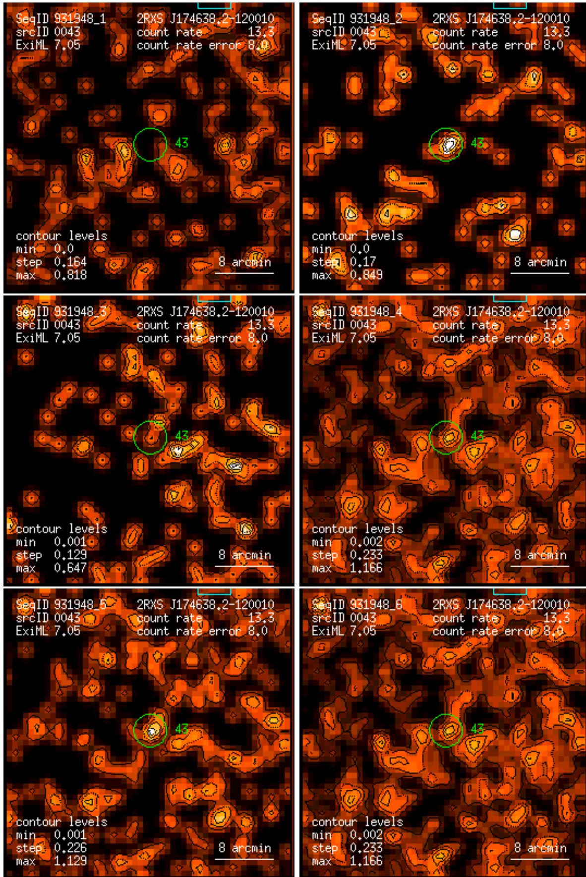
Figure 43: RASS 931948: detection 0043: band rate images, Gaussian filter: (1) PSPC channels 11 – 41, (2) 52 – 90, (3) 91 – 201, (4) 11 – 235, (5) 52 – 201, (6) 11 – 201. Broad band rates in counts/ks. Band rate contour levels in counts/ks/arcmin 2 .
