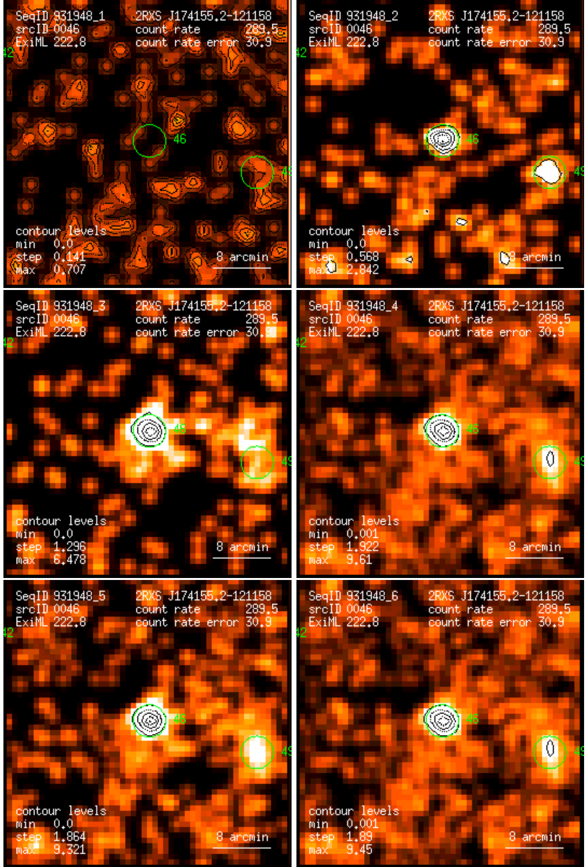
Figure 46: RASS 931948: detection 0046: band rate images, Gaussian filter: (1) PSPC channels 11 – 41, (2) 52 – 90, (3) 91 – 201, (4) 11 – 235, (5) 52 – 201, (6) 11 – 201. Broad band rates in counts/ks. Band rate contour levels in counts/ks/arcmin 2 .
