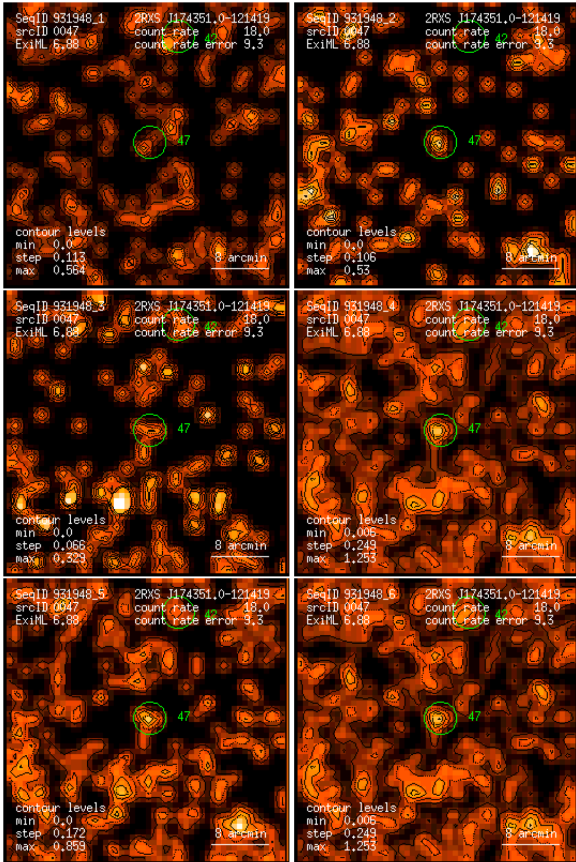
Figure 47: RASS 931948: detection 0047: band rate images, Gaussian filter: (1) PSPC channels 11 – 41, (2) 52 – 90, (3) 91 – 201, (4) 11 – 235, (5) 52 – 201, (6) 11 – 201. Broad band rates in counts/ks. Band rate contour levels in counts/ks/arcmin 2 .
