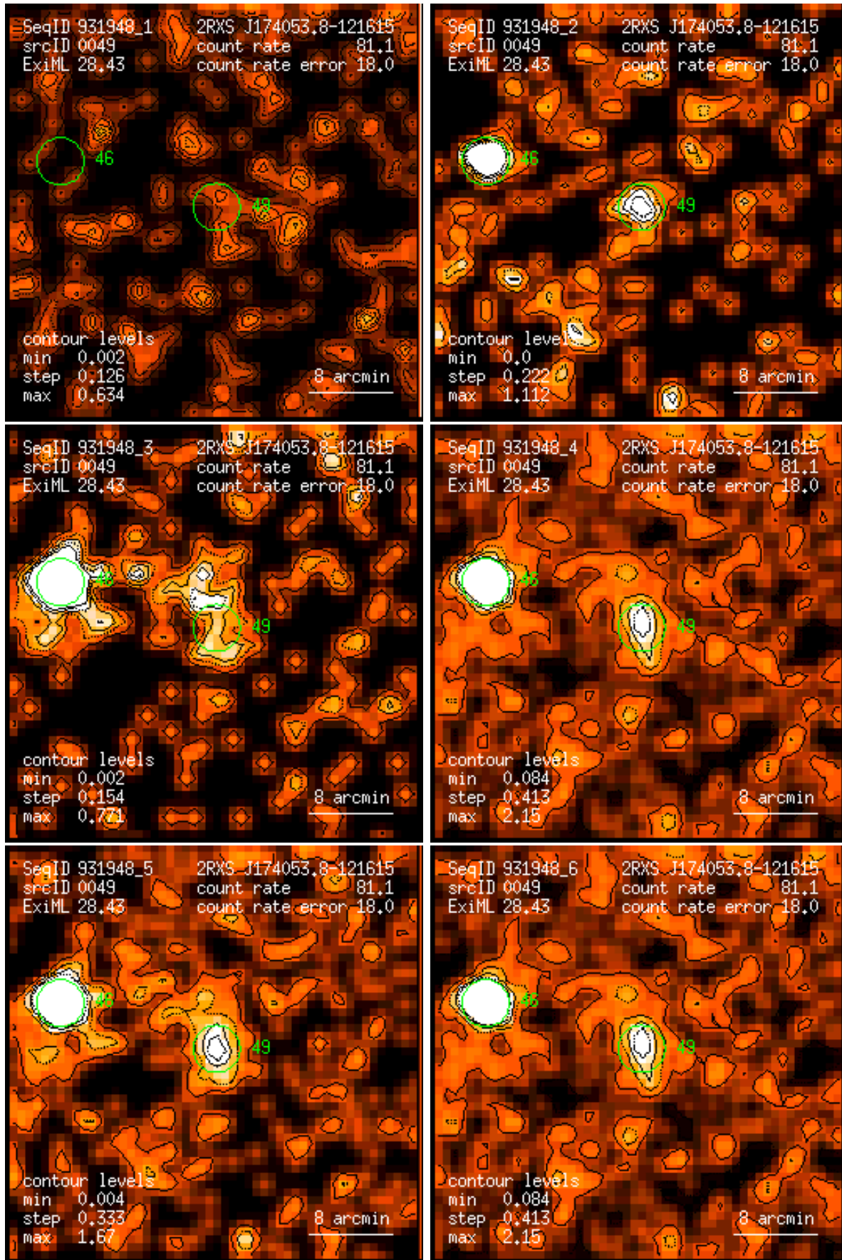
Figure 49: RASS 931948: detection 0049: band rate images, Gaussian filter: (1) PSPC channels 11 – 41, (2) 52 – 90, (3) 91 – 201, (4) 11 – 235, (5) 52 – 201, (6) 11 – 201. Broad band rates in counts/ks. Band rate contour levels in counts/ks/arcmin 2 .
