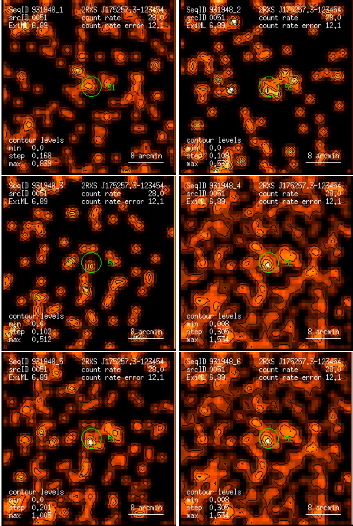
Figure 51: RASS 931948: detection 0051: band rate images, Gaussian filter: (1) PSPC channels 11 – 41, (2) 52 – 90, (3) 91 – 201, (4) 11 – 235, (5) 52 – 201, (6) 11 – 201. Broad band rates in counts/ks. Band rate contour levels in counts/ks/arcmin 2 .
