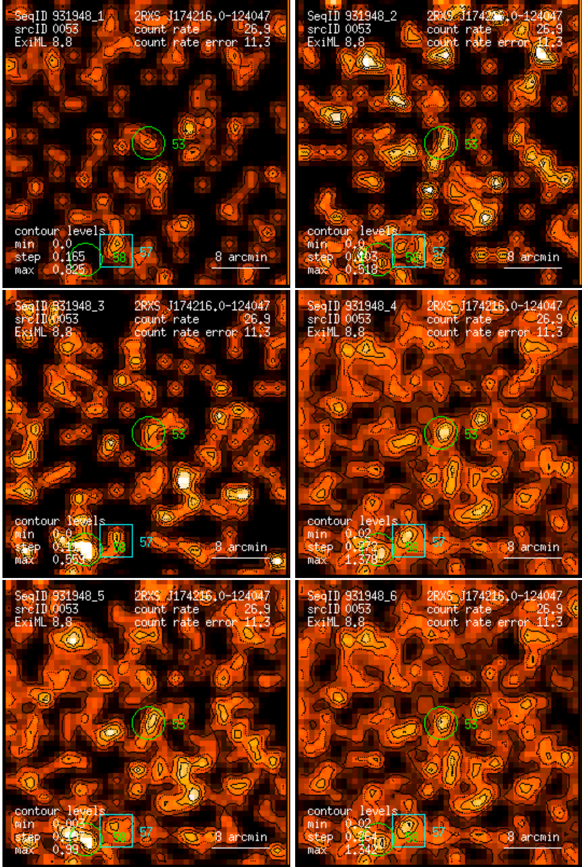
Figure 53: RASS 931948: detection 0053: band rate images, Gaussian filter: (1) PSPC channels 11 – 41, (2) 52 – 90, (3) 91 – 201, (4) 11 – 235, (5) 52 – 201, (6) 11 – 201. Broad band rates in counts/ks. Band rate contour levels in counts/ks/arcmin 2 .
