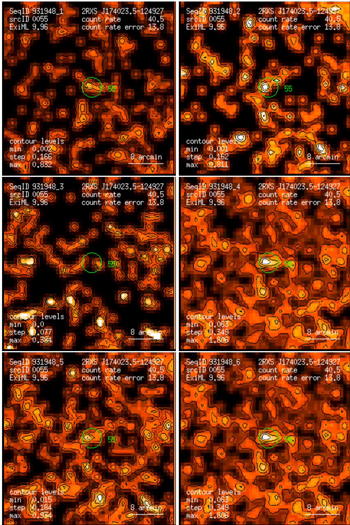
Figure 55: RASS 931948: detection 0055: band rate images, Gaussian filter: (1) PSPC channels 11 – 41, (2) 52 – 90, (3) 91 – 201, (4) 11 – 235, (5) 52 – 201, (6) 11 – 201. Broad band rates in counts/ks. Band rate contour levels in counts/ks/arcmin 2 .
