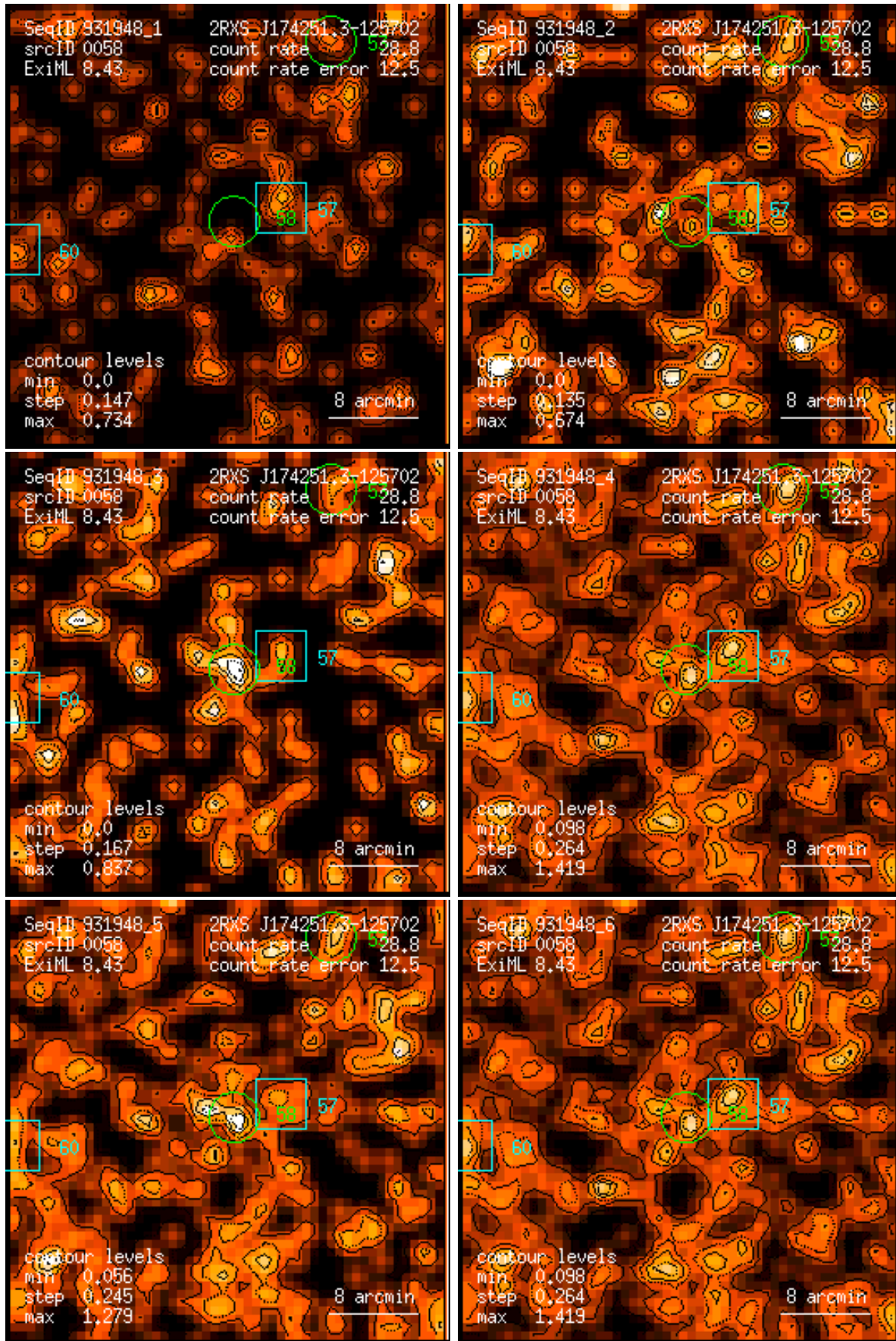
Figure 58: RASS 931948: detection 0058: band rate images, Gaussian filter: (1) PSPC channels 11 – 41, (2) 52 – 90, (3) 91 – 201, (4) 11 – 235, (5) 52 – 201, (6) 11 – 201. Broad band rates in counts/ks. Band rate contour levels in counts/ks/arcmin 2 .
