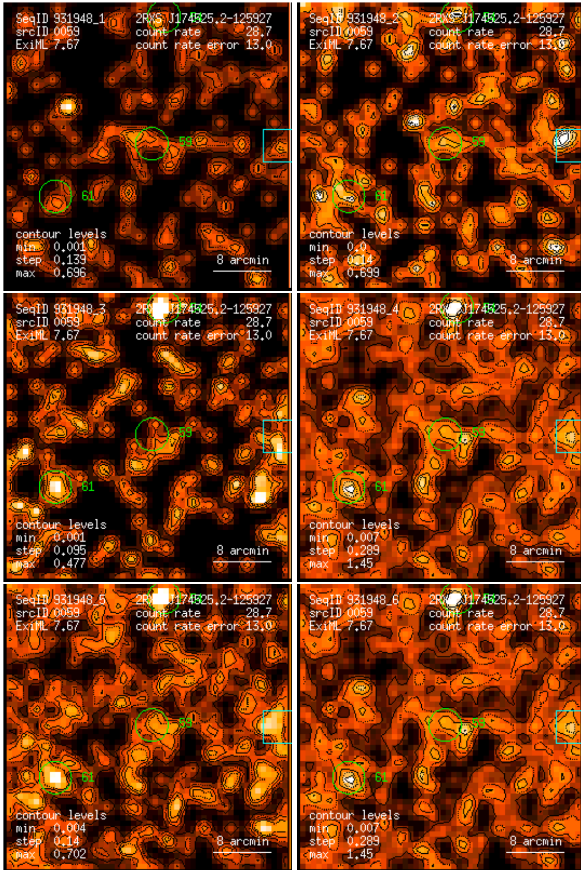
Figure 59: RASS 931948: detection 0059: band rate images, Gaussian filter: (1) PSPC channels 11 – 41, (2) 52 – 90, (3) 91 – 201, (4) 11 – 235, (5) 52 – 201, (6) 11 – 201. Broad band rates in counts/ks. Band rate contour levels in counts/ks/arcmin 2 .
