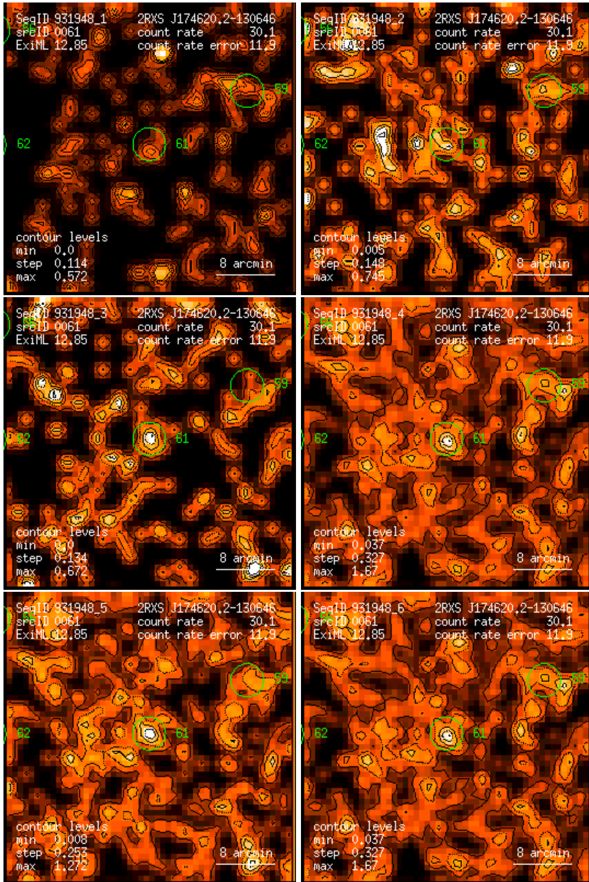
Figure 61: RASS 931948: detection 0061: band rate images, Gaussian filter: (1) PSPC channels 11 – 41, (2) 52 – 90, (3) 91 – 201, (4) 11 – 235, (5) 52 – 201, (6) 11 – 201. Broad band rates in counts/ks. Band rate contour levels in counts/ks/arcmin 2 .
