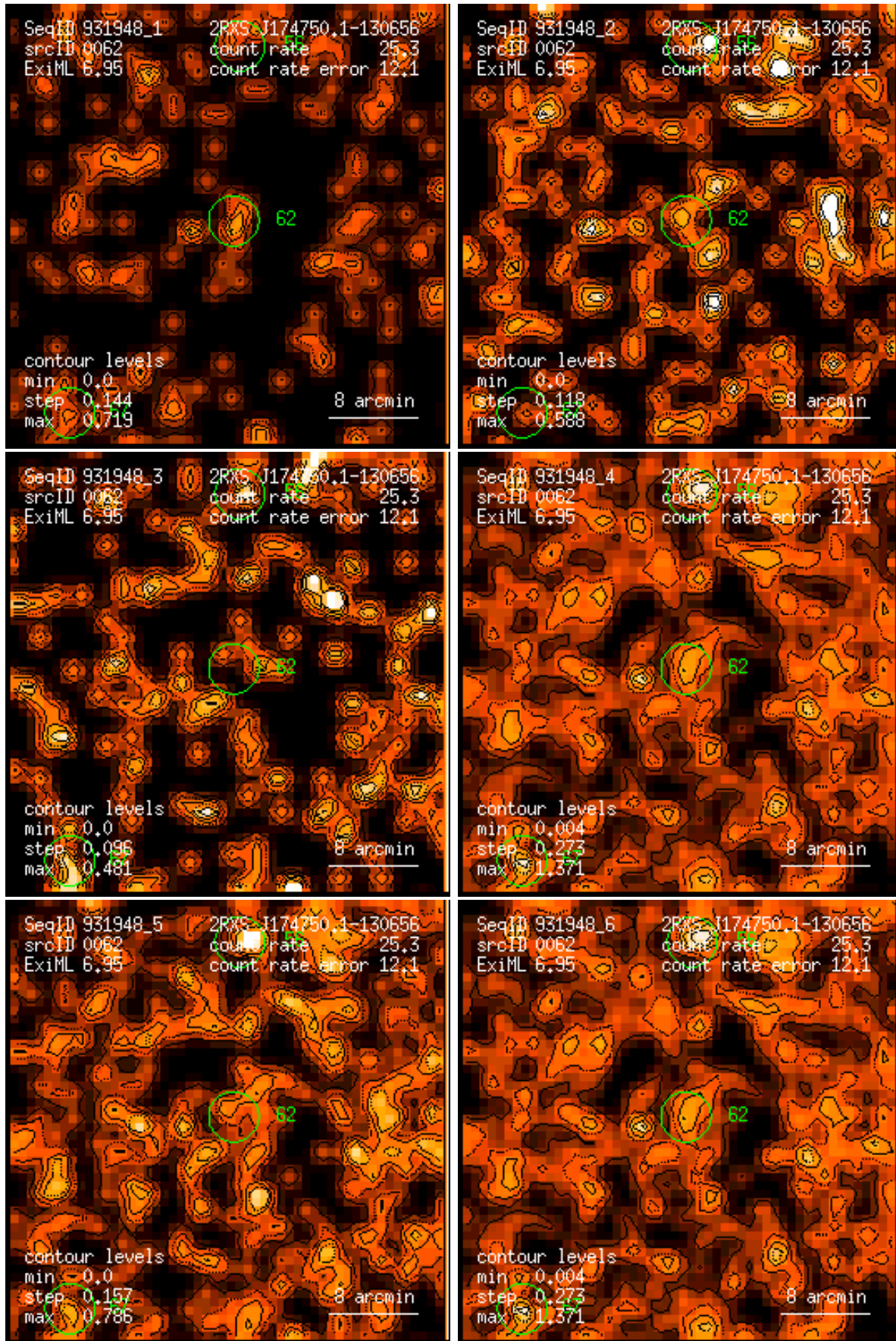
Figure 62: RASS 931948: detection 0062: band rate images, Gaussian filter: (1) PSPC channels 11 – 41, (2) 52 – 90, (3) 91 – 201, (4) 11 – 235, (5) 52 – 201, (6) 11 – 201. Broad band rates in counts/ks. Band rate contour levels in counts/ks/arcmin 2 .
