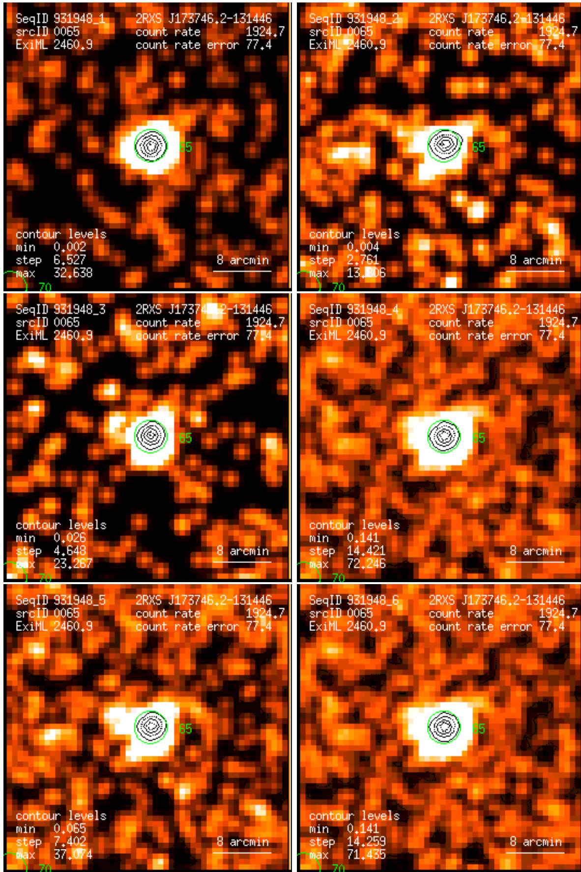
Figure 65: RASS 931948: detection 0065: band rate images, Gaussian filter: (1) PSPC channels 11 – 41, (2) 52 – 90, (3) 91 – 201, (4) 11 – 235, (5) 52 – 201, (6) 11 – 201. Broad band rates in counts/ks. Band rate contour levels in counts/ks/arcmin 2 .
