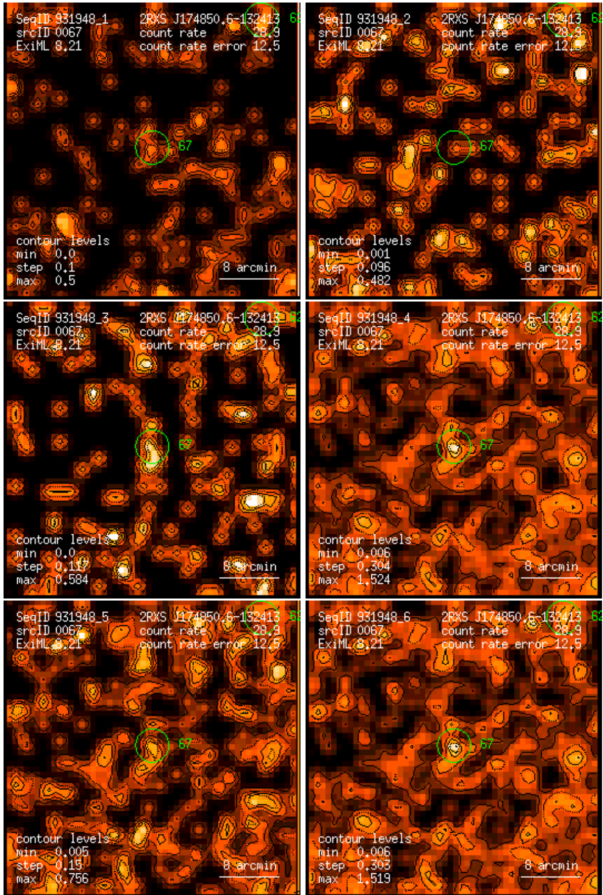
Figure 67: RASS 931948: detection 0067: band rate images, Gaussian filter: (1) PSPC channels 11 – 41, (2) 52 – 90, (3) 91 – 201, (4) 11 – 235, (5) 52 – 201, (6) 11 – 201. Broad band rates in counts/ks. Band rate contour levels in counts/ks/arcmin 2 .
