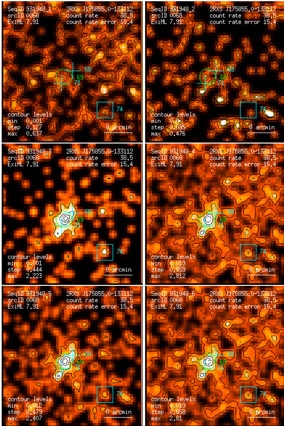
Figure 68: RASS 931948: detection 0068: band rate images, Gaussian filter: (1) PSPC channels 11 – 41, (2) 52 – 90, (3) 91 – 201, (4) 11 – 235, (5) 52 – 201, (6) 11 – 201. Broad band rates in counts/ks. Band rate contour levels in counts/ks/arcmin 2 .
