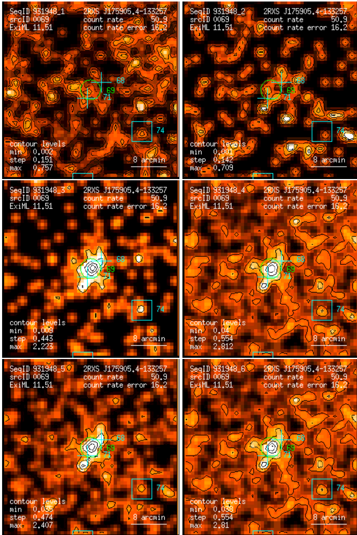
Figure 69: RASS 931948: detection 0069: band rate images, Gaussian filter: (1) PSPC channels 11 – 41, (2) 52 – 90, (3) 91 – 201, (4) 11 – 235, (5) 52 – 201, (6) 11 – 201. Broad band rates in counts/ks. Band rate contour levels in counts/ks/arcmin 2 .
