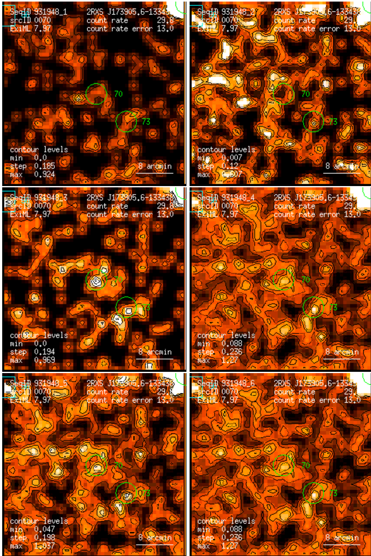
Figure 70: RASS 931948: detection 0070: band rate images, Gaussian filter: (1) PSPC channels 11 – 41, (2) 52 – 90, (3) 91 – 201, (4) 11 – 235, (5) 52 – 201, (6) 11 – 201. Broad band rates in counts/ks. Band rate contour levels in counts/ks/arcmin 2 .
