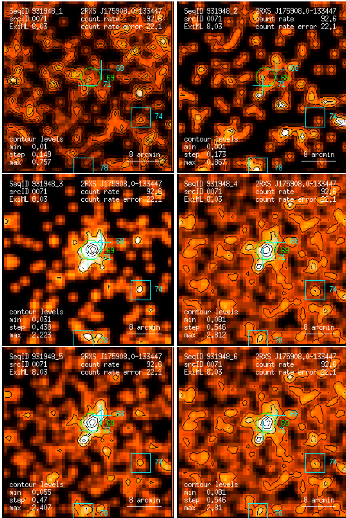
Figure 71: RASS 931948: detection 0071: band rate images, Gaussian filter: (1) PSPC channels 11 – 41, (2) 52 – 90, (3) 91 – 201, (4) 11 – 235, (5) 52 – 201, (6) 11 – 201. Broad band rates in counts/ks. Band rate contour levels in counts/ks/arcmin 2 .
