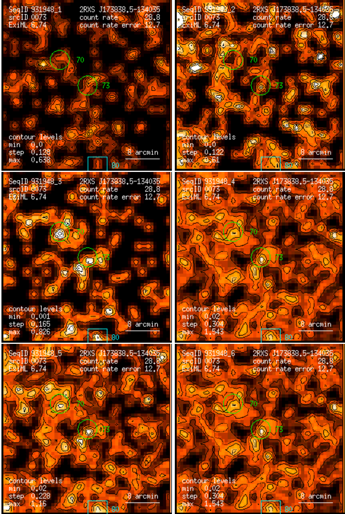
Figure 73: RASS 931948: detection 0073: band rate images, Gaussian filter: (1) PSPC channels 11 – 41, (2) 52 – 90, (3) 91 – 201, (4) 11 – 235, (5) 52 – 201, (6) 11 – 201. Broad band rates in counts/ks. Band rate contour levels in counts/ks/arcmin 2 .
