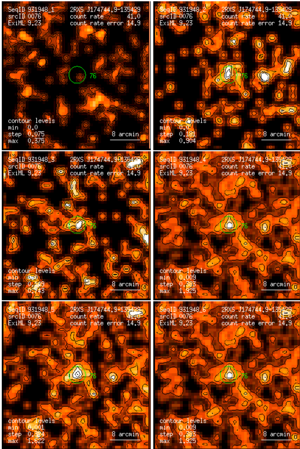
Figure 76: RASS 931948: detection 0076: band rate images, Gaussian filter: (1) PSPC channels 11 – 41, (2) 52 – 90, (3) 91 – 201, (4) 11 – 235, (5) 52 – 201, (6) 11 – 201. Broad band rates in counts/ks. Band rate contour levels in counts/ks/arcmin 2 .
