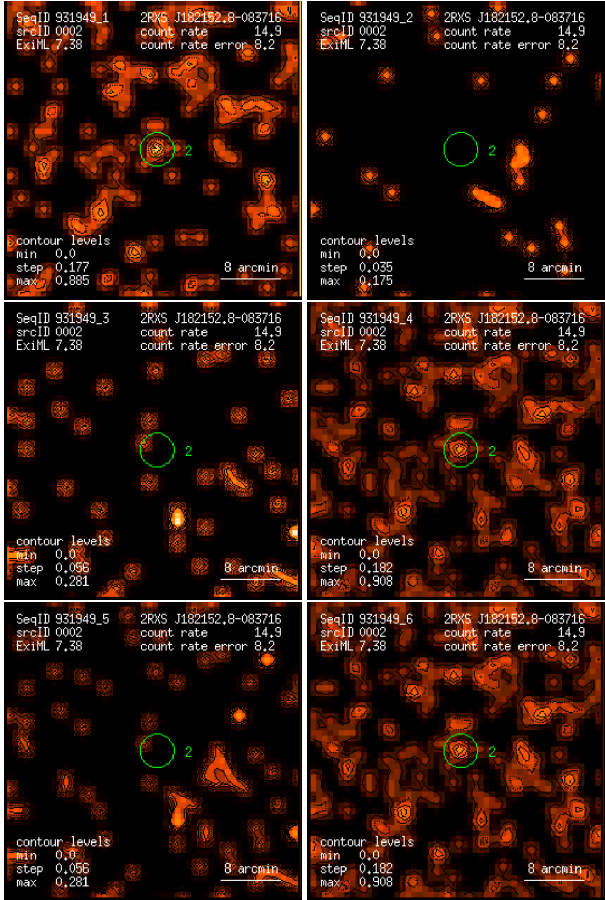
Figure 2: RASS 931949: detection 0002: band rate images, Gaussian filter: (1) PSPC channels 11 – 41, (2) 52 – 90, (3) 91 – 201, (4) 11 – 235, (5) 52 – 201, (6) 11 – 201. Broad band rates in counts/ks. Band rate contour levels in counts/ks/arcmin 2 .
