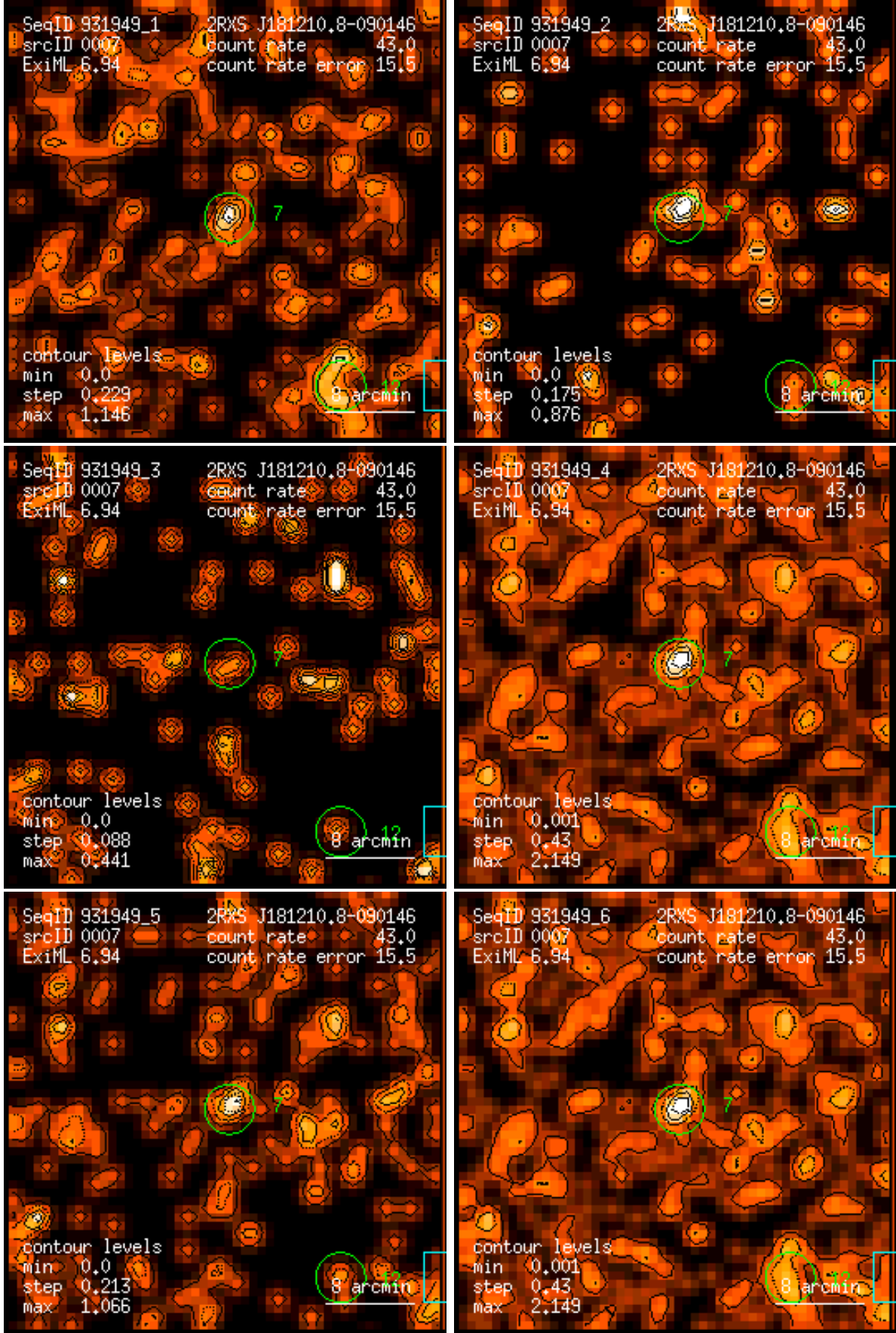
Figure 7: RASS 931949: detection 0007: band rate images, Gaussian filter: (1) PSPC channels 11 – 41, (2) 52 – 90, (3) 91 – 201, (4) 11 – 235, (5) 52 – 201, (6) 11 – 201. Broad band rates in counts/ks. Band rate contour levels in counts/ks/arcmin 2 .
