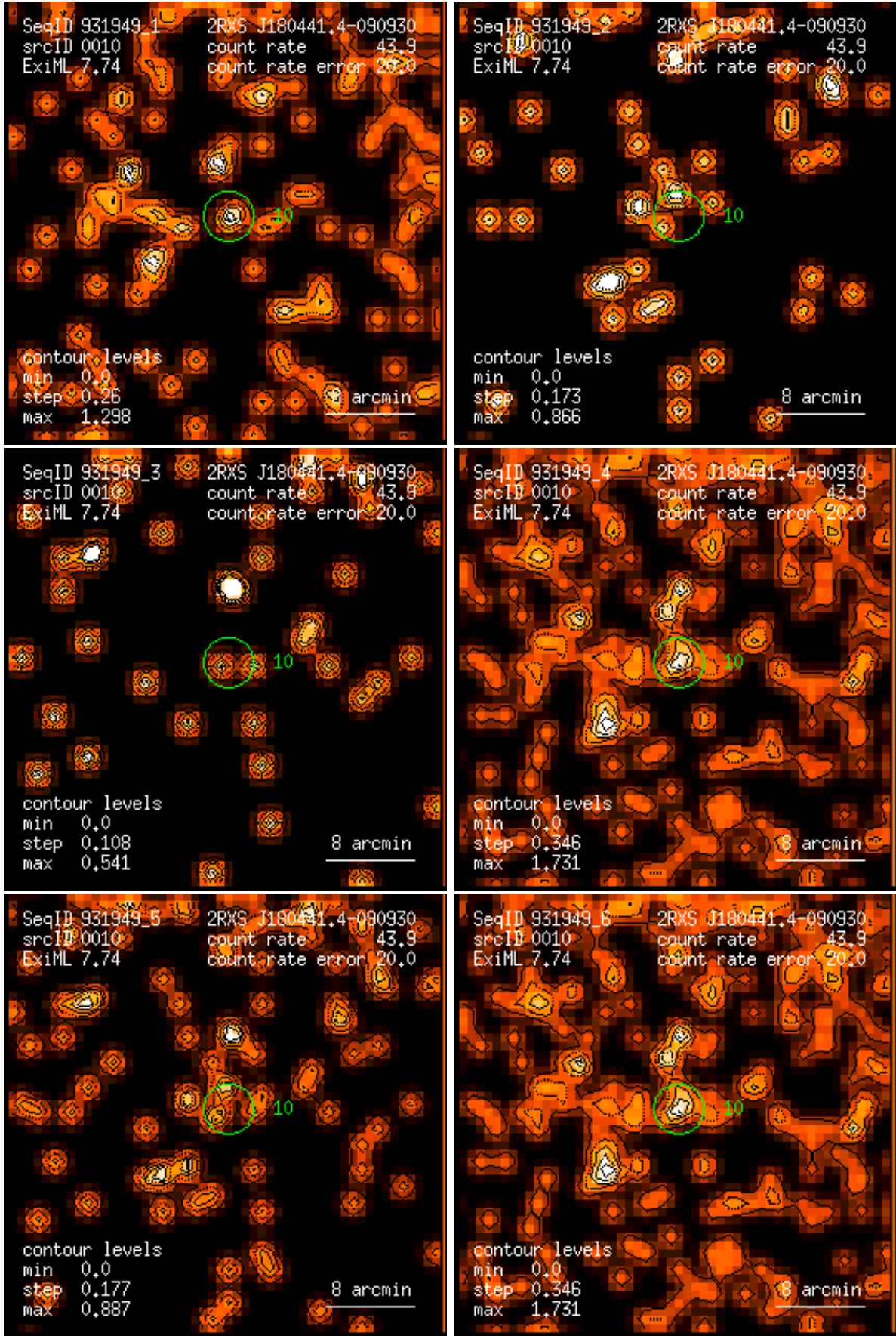
Figure 10: RASS 931949: detection 0010: band rate images, Gaussian filter: (1) PSPC channels 11 – 41, (2) 52 – 90, (3) 91 – 201, (4) 11 – 235, (5) 52 – 201, (6) 11 – 201. Broad band rates in counts/ks. Band rate contour levels in counts/ks/arcmin 2 .
