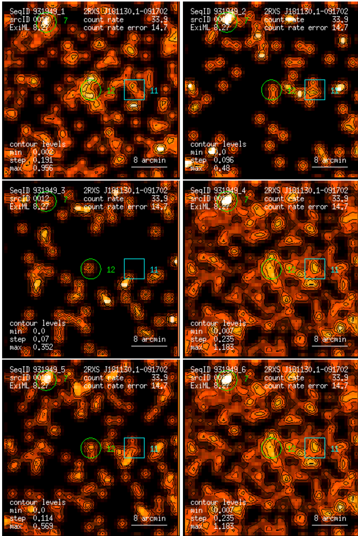
Figure 12: RASS 931949: detection 0012: band rate images, Gaussian filter: (1) PSPC channels 11 – 41, (2) 52 – 90, (3) 91 – 201, (4) 11 – 235, (5) 52 – 201, (6) 11 – 201. Broad band rates in counts/ks. Band rate contour levels in counts/ks/arcmin 2 .
