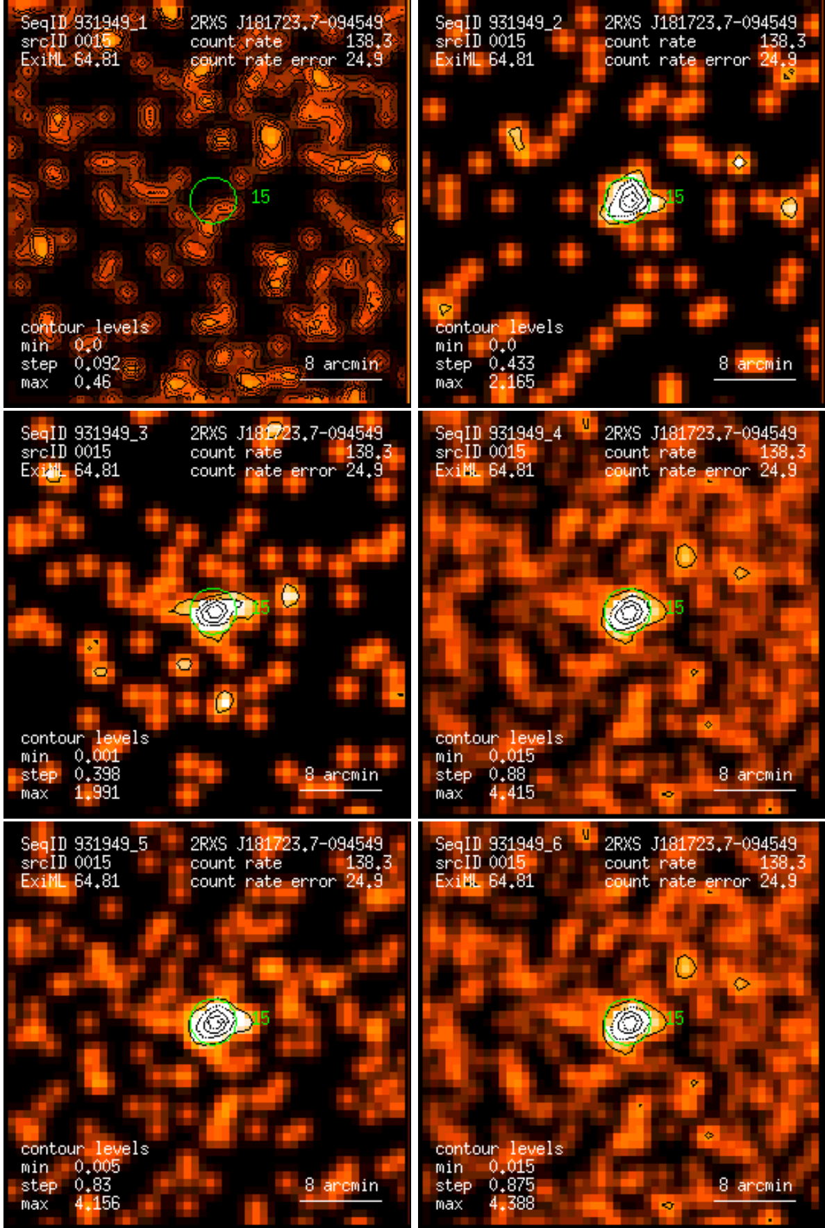
Figure 15: RASS 931949: detection 0015: band rate images, Gaussian filter: (1) PSPC channels 11 – 41, (2) 52 – 90, (3) 91 – 201, (4) 11 – 235, (5) 52 – 201, (6) 11 – 201. Broad band rates in counts/ks. Band rate contour levels in counts/ks/arcmin 2 .
