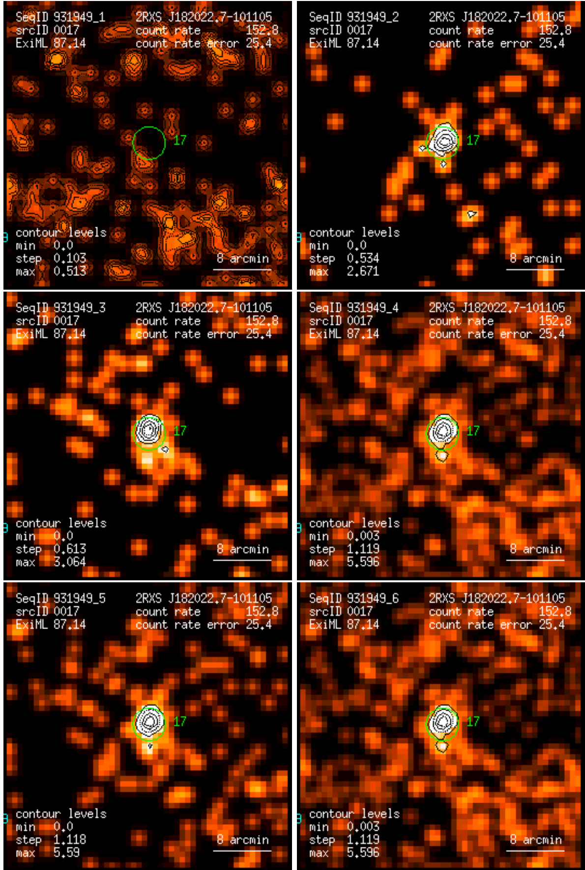
Figure 17: RASS 931949: detection 0017: band rate images, Gaussian filter: (1) PSPC channels 11 – 41, (2) 52 – 90, (3) 91 – 201, (4) 11 – 235, (5) 52 – 201, (6) 11 – 201. Broad band rates in counts/ks. Band rate contour levels in counts/ks/arcmin 2 .
