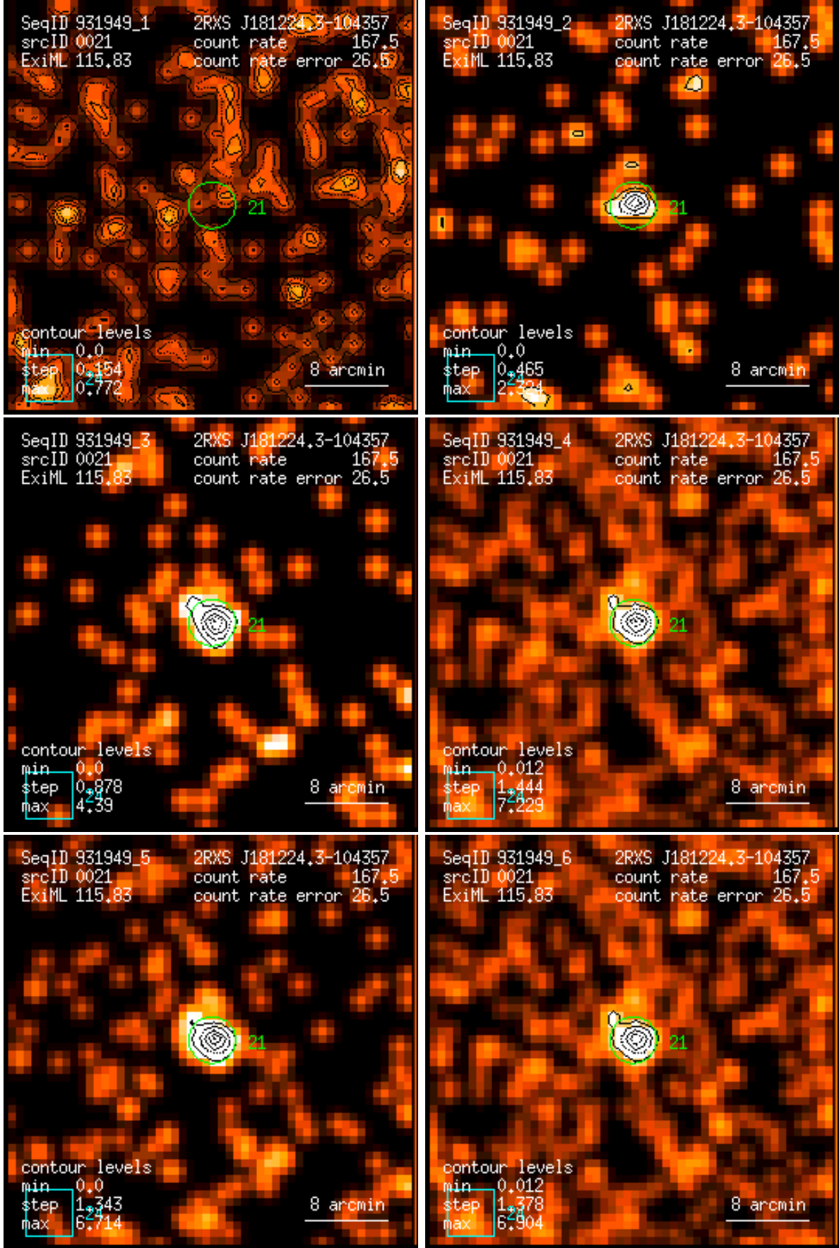
Figure 21: RASS 931949: detection 0021: band rate images, Gaussian filter: (1) PSPC channels 11 – 41, (2) 52 – 90, (3) 91 – 201, (4) 11 – 235, (5) 52 – 201, (6) 11 – 201. Broad band rates in counts/ks. Band rate contour levels in counts/ks/arcmin 2 .
