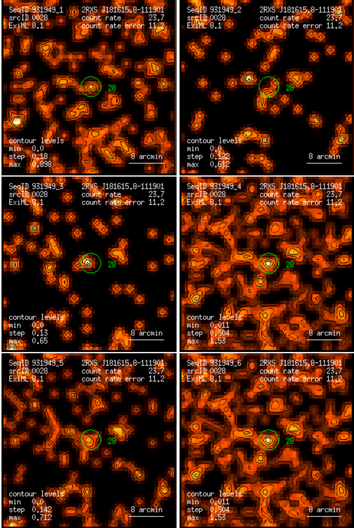
Figure 28: RASS 931949: detection 0028: band rate images, Gaussian filter: (1) PSPC channels 11 – 41, (2) 52 – 90, (3) 91 – 201, (4) 11 – 235, (5) 52 – 201, (6) 11 – 201. Broad band rates in counts/ks. Band rate contour levels in counts/ks/arcmin 2 .
