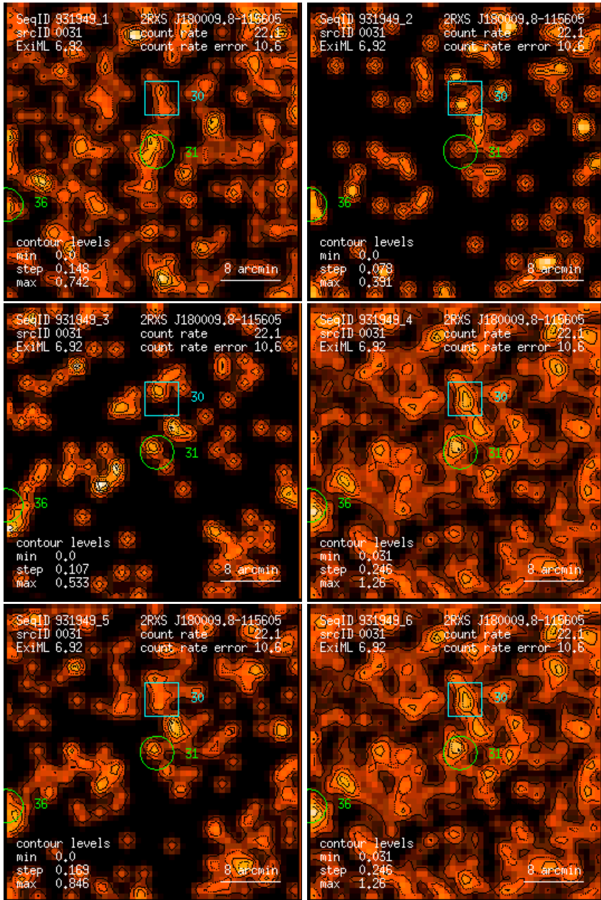
Figure 31: RASS 931949: detection 0031: band rate images, Gaussian filter: (1) PSPC channels 11 – 41, (2) 52 – 90, (3) 91 – 201, (4) 11 – 235, (5) 52 – 201, (6) 11 – 201. Broad band rates in counts/ks. Band rate contour levels in counts/ks/arcmin 2 .
