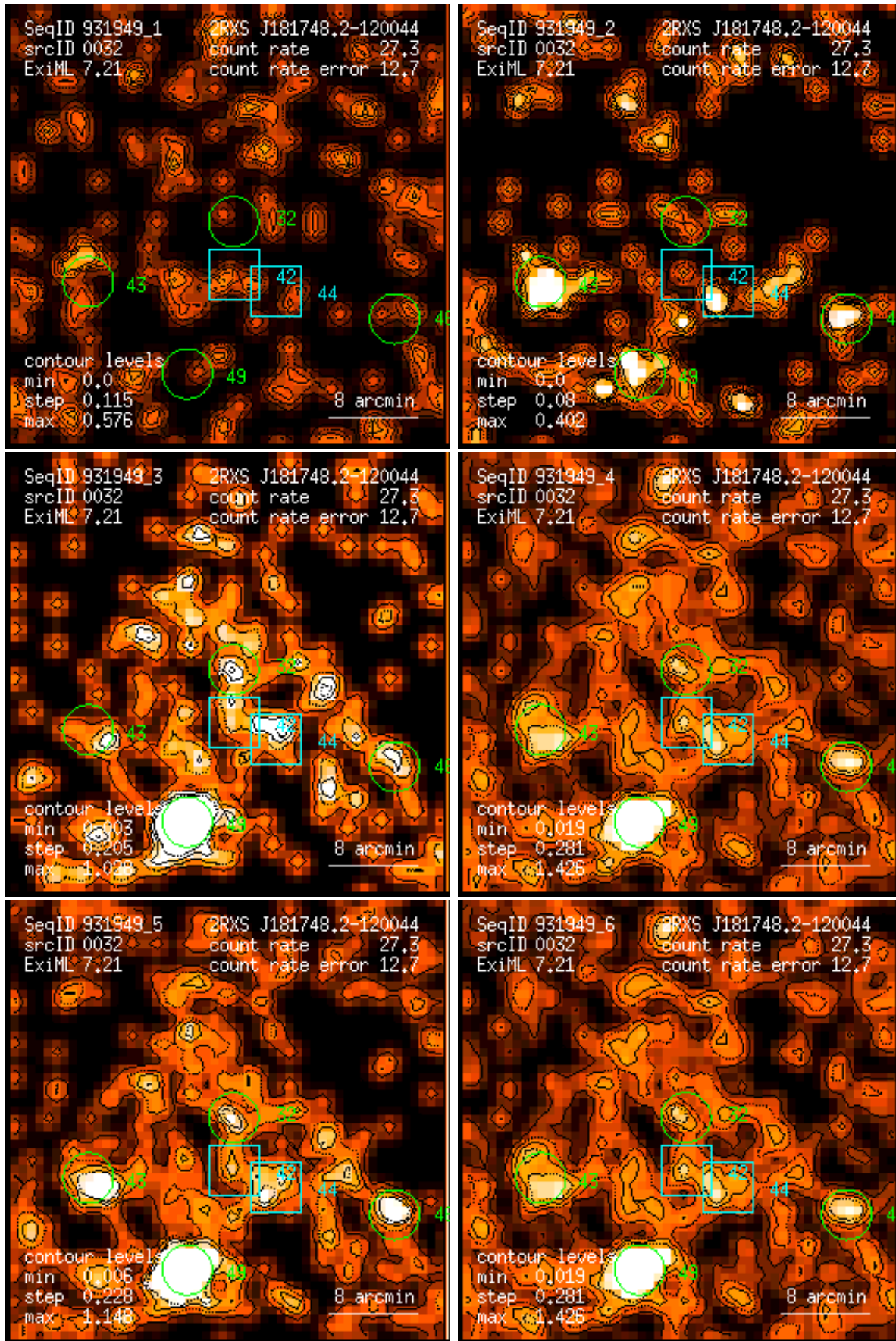
Figure 32: RASS 931949: detection 0032: band rate images, Gaussian filter: (1) PSPC channels 11 – 41, (2) 52 – 90, (3) 91 – 201, (4) 11 – 235, (5) 52 – 201, (6) 11 – 201. Broad band rates in counts/ks. Band rate contour levels in counts/ks/arcmin 2 .
