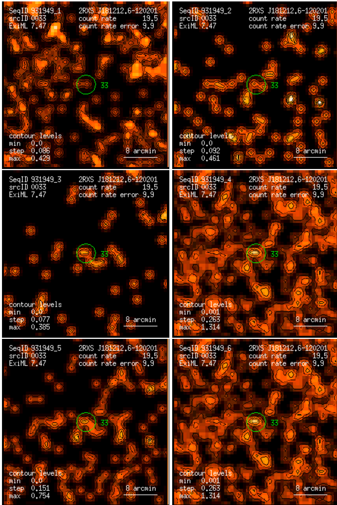
Figure 33: RASS 931949: detection 0033: band rate images, Gaussian filter: (1) PSPC channels 11 – 41, (2) 52 – 90, (3) 91 – 201, (4) 11 – 235, (5) 52 – 201, (6) 11 – 201. Broad band rates in counts/ks. Band rate contour levels in counts/ks/arcmin 2 .
