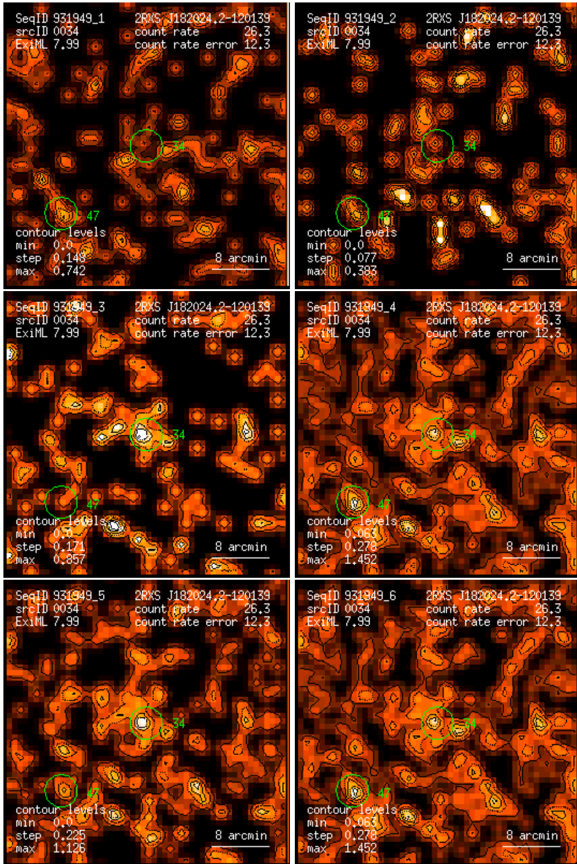
Figure 34: RASS 931949: detection 0034: band rate images, Gaussian filter: (1) PSPC channels 11 – 41, (2) 52 – 90, (3) 91 – 201, (4) 11 – 235, (5) 52 – 201, (6) 11 – 201. Broad band rates in counts/ks. Band rate contour levels in counts/ks/arcmin 2 .
