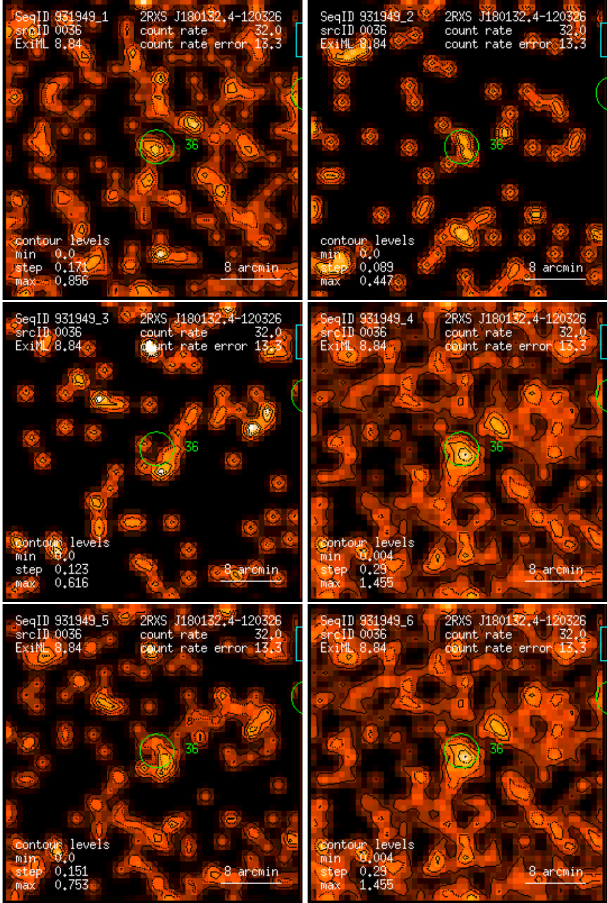
Figure 36: RASS 931949: detection 0036: band rate images, Gaussian filter: (1) PSPC channels 11 – 41, (2) 52 – 90, (3) 91 – 201, (4) 11 – 235, (5) 52 – 201, (6) 11 – 201. Broad band rates in counts/ks. Band rate contour levels in counts/ks/arcmin 2 .
